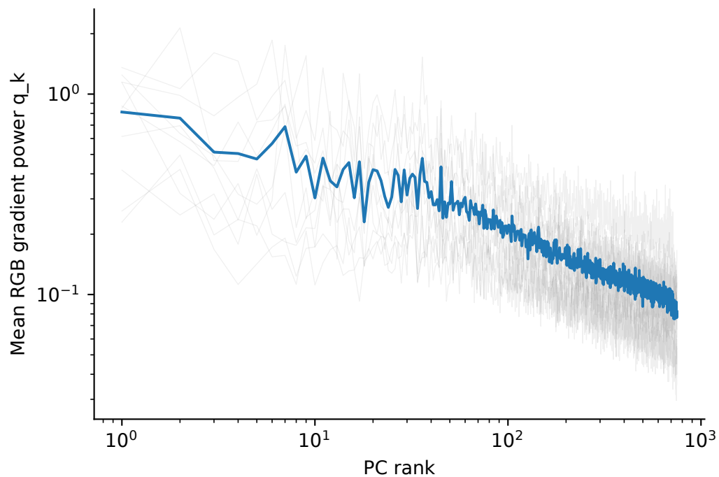
clipag_vitb32 .transformer.resblocks.ResidualAttentionBlock8 | 774 training images Geometry pilot: 10 seeds images, 750 PCs; empirical spectrum
