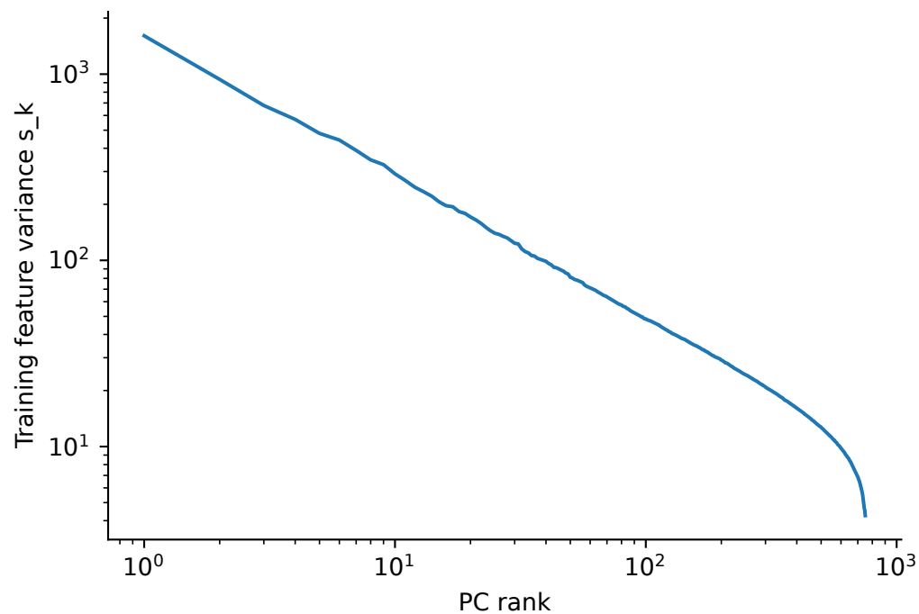
resnet50_robust .layer4.Bottleneck1 | 774 training images Geometry pilot: 2 images, 750 PCs; empirical spectrum
