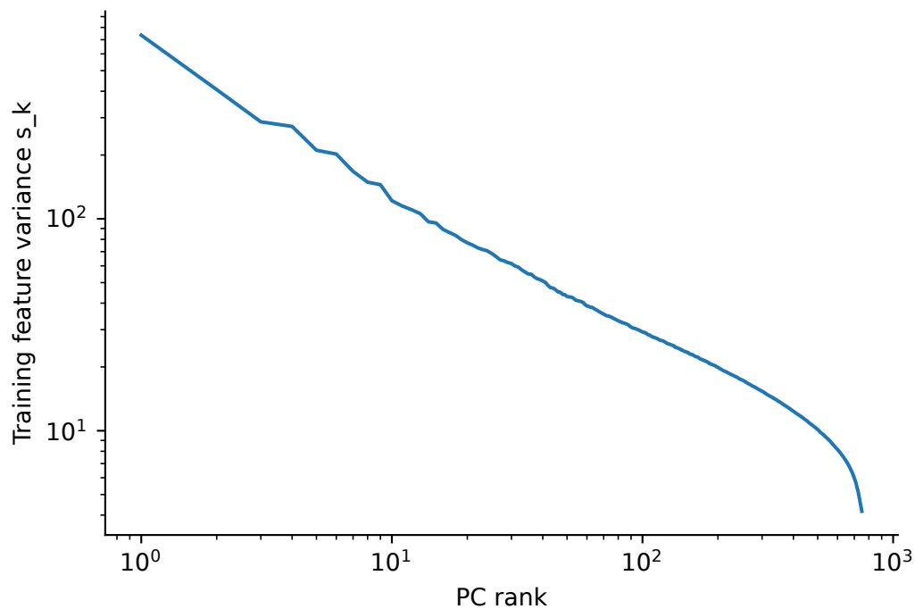
resnet50 .layer4.Bottleneck1 | 774 training images Geometry pilot: 10 seeds images, 750 PCs; empirical spectrum
