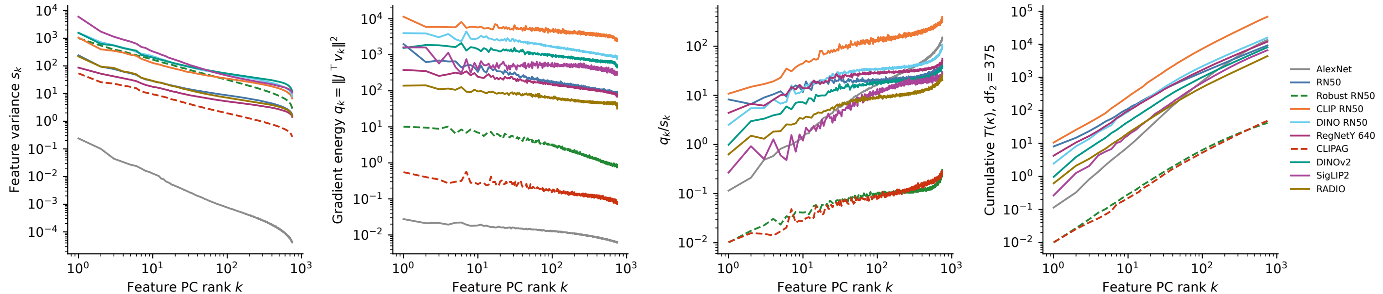
PC-resolved gradient geometry of the ten encoding models: site-weighted log-mean over layer geometries (dashed: adversarially trained; matched \text{df}_2=375 )
