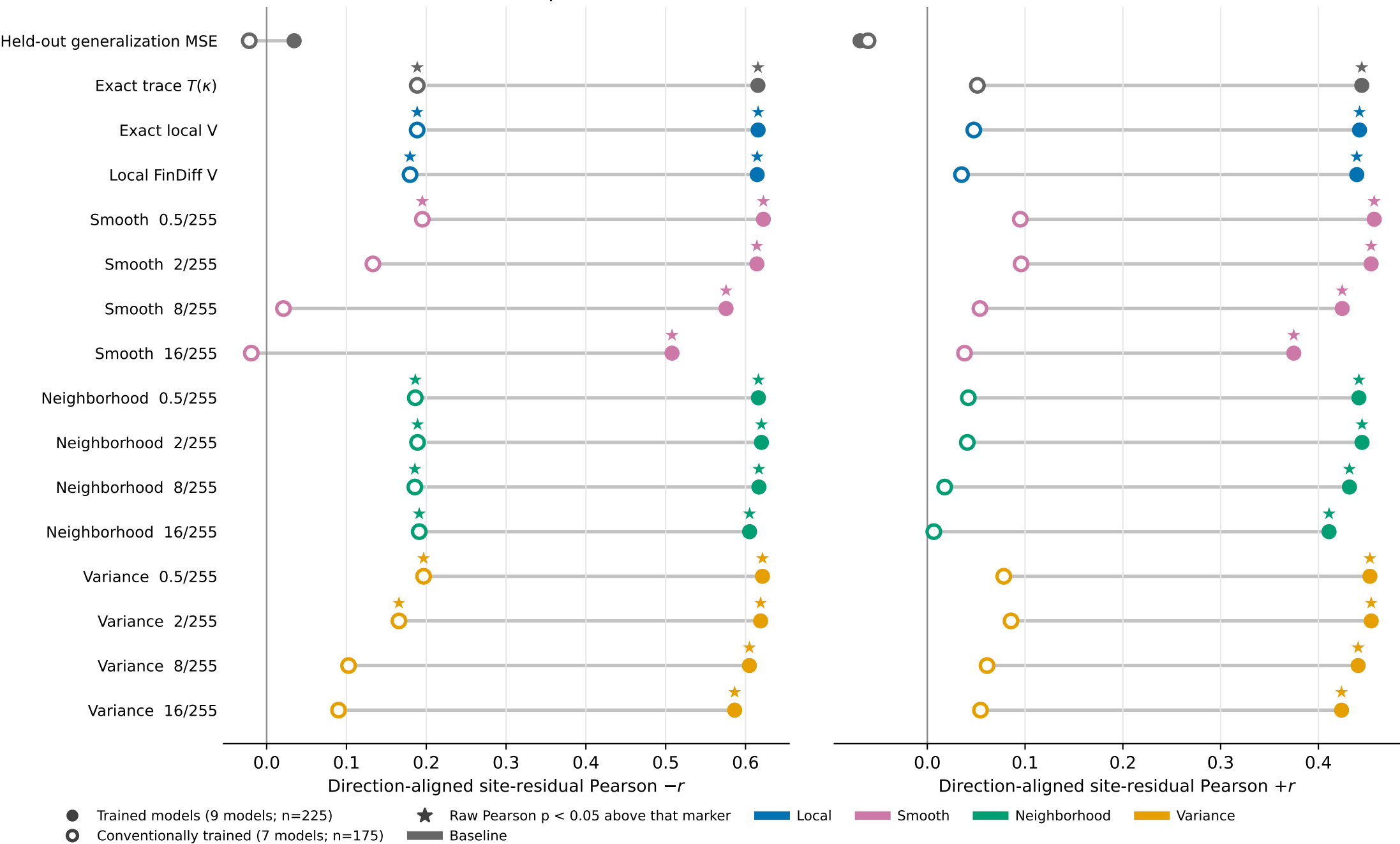
Benchmark of control-geometry predictors of biological outcomes Control session; one train-anchor site affine shared across all models; site means removed; stars: Raw Pearson p < 0.05
