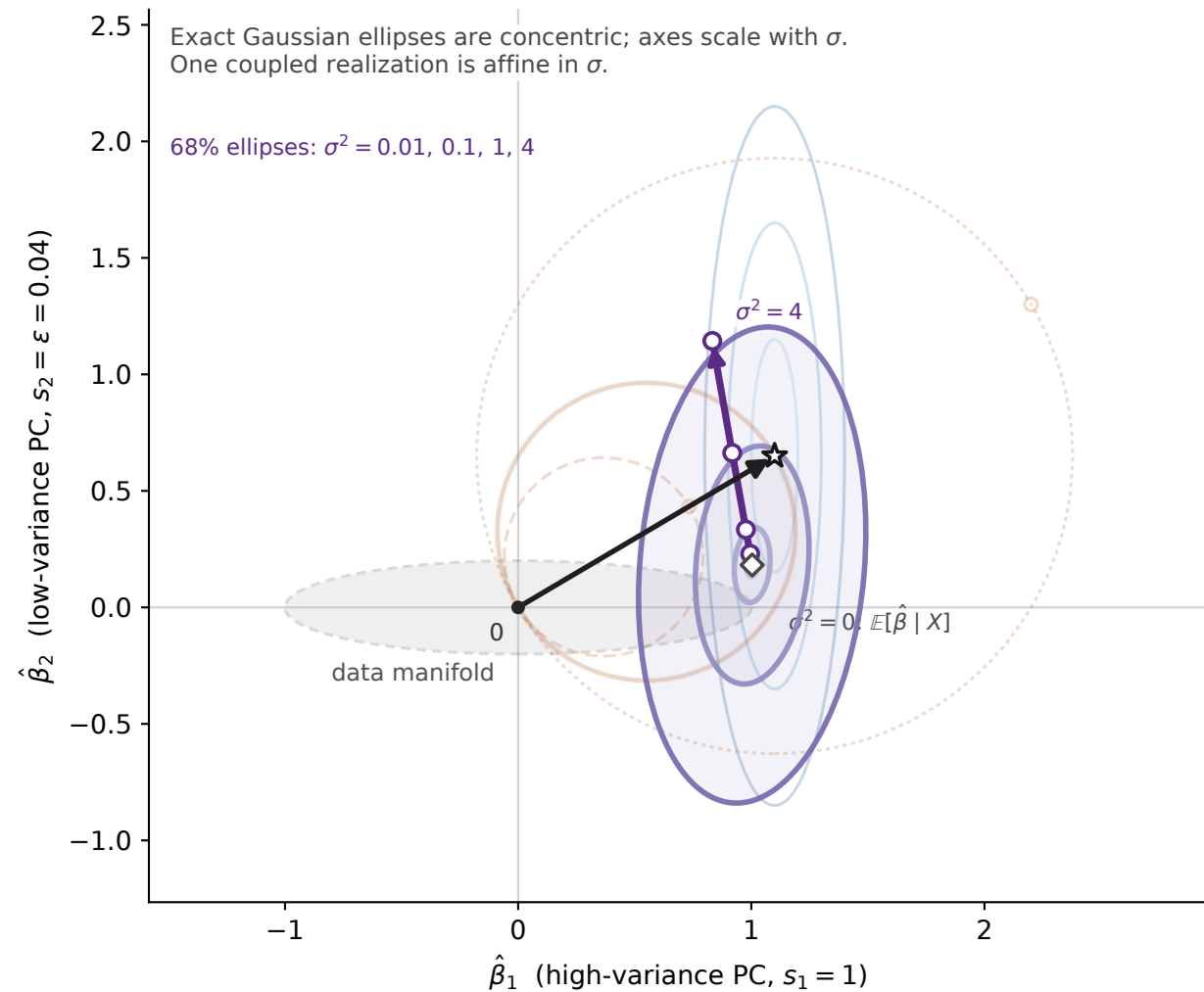
a Fixed \lambda = 0.05 ( \kappa = 0.0518 ); vary \sigma^2 on log grid
