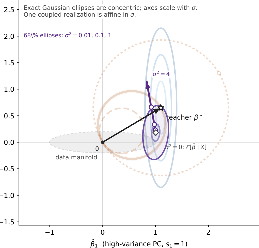
a Fixed \lambda = 0.05 ( \kappa = 0.0518 ); vary \sigma^2 on log grid
