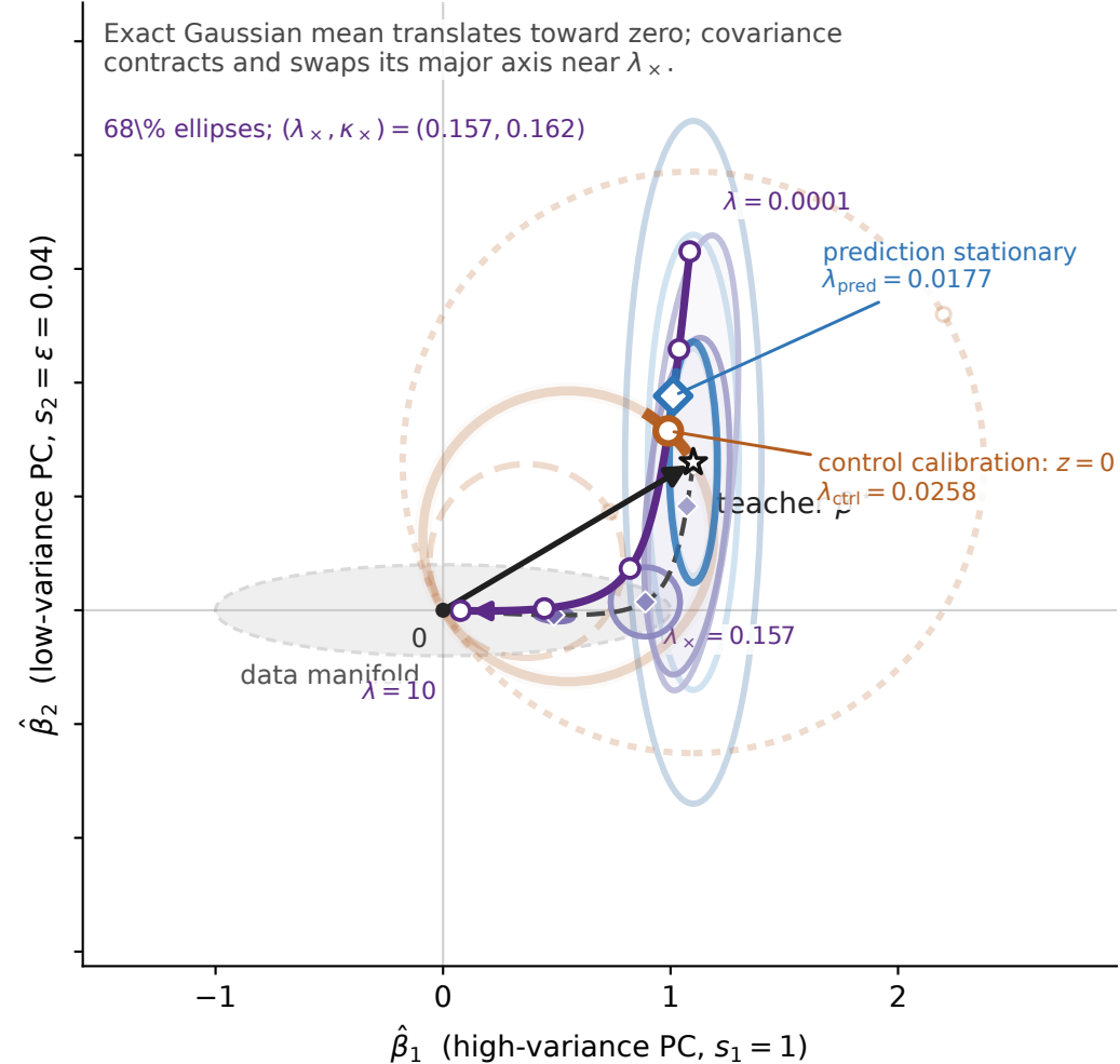
b Fixed \sigma^2 = 0.5 ; vary \lambda/\kappa on log grid
