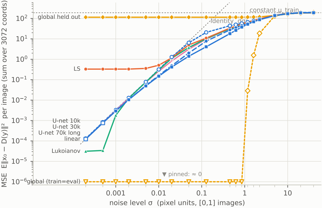
MSE vs noise, FFHQ 32x32
