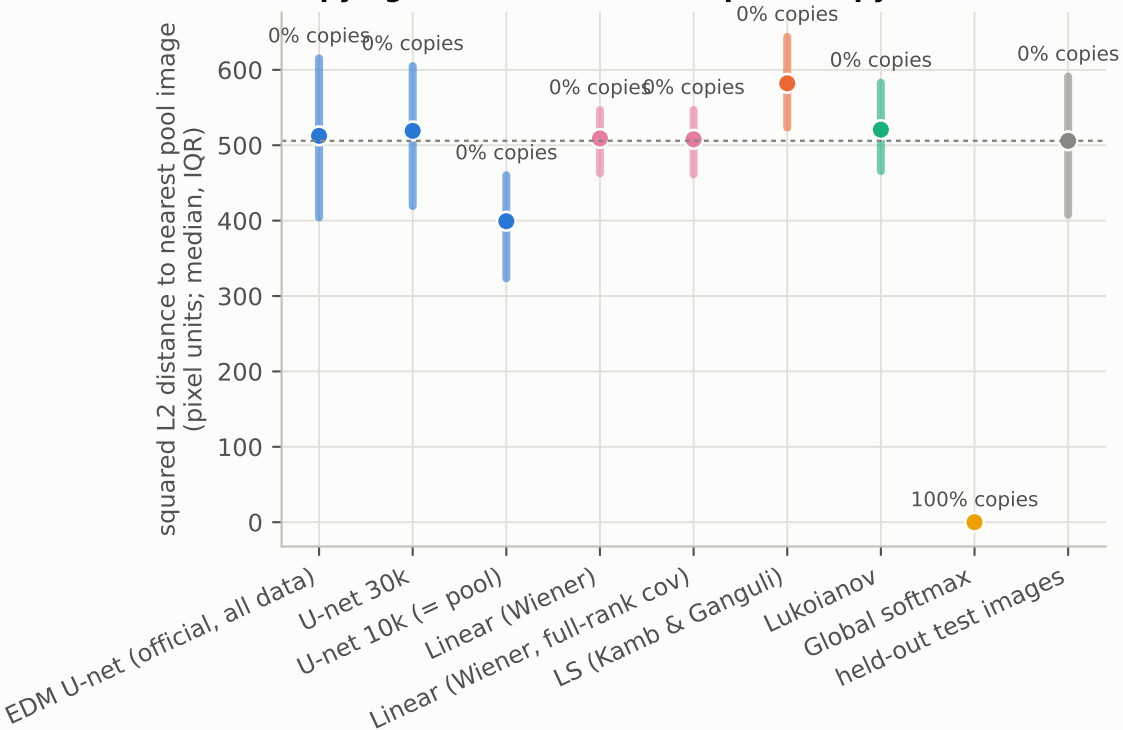
Copying: distance to the 10k pool (copy = d_1/d_2 < 1/3 )
