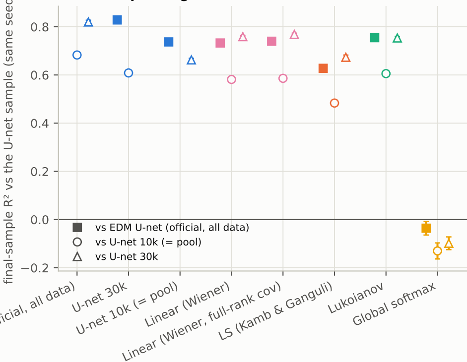
Final samples: agreement with each U-net
