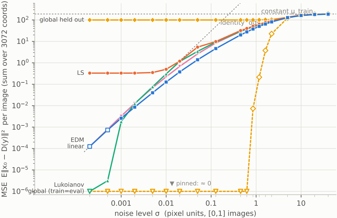
MSE vs noise, CIFAR-10
