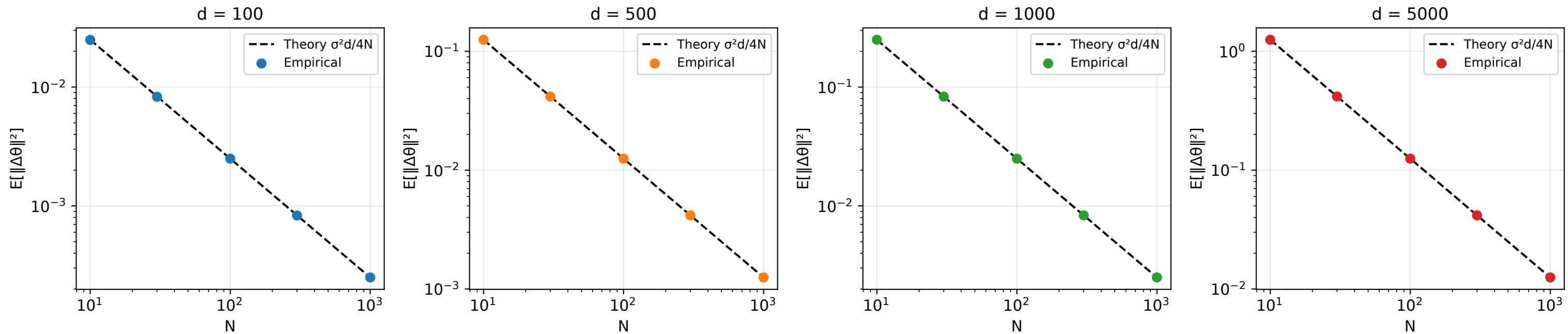
Exp 1a: One-step drift variance vs N
