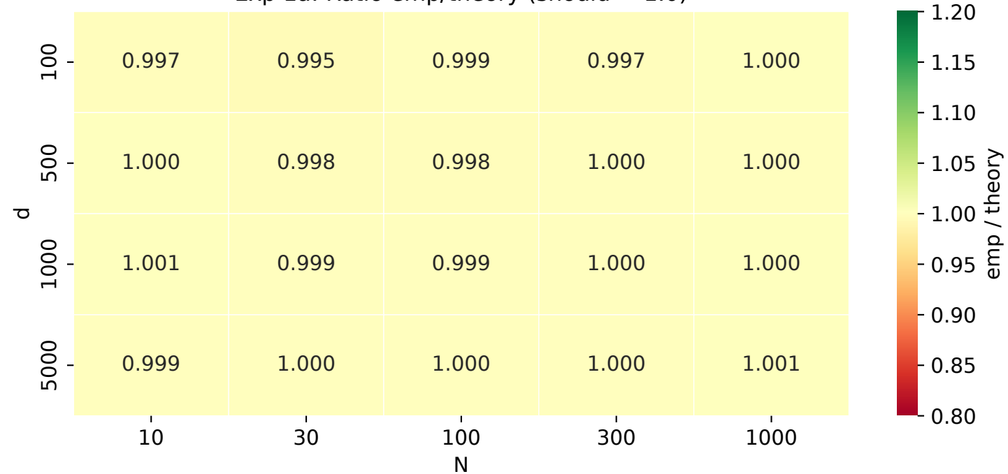
Exp 1a: Ratio emp/theory (should = 1.0)
