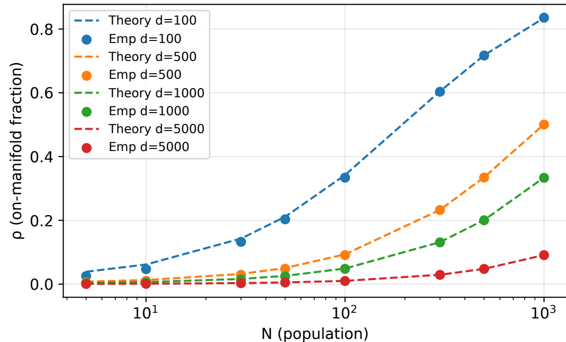
Exp 2b: \rho vs population N
