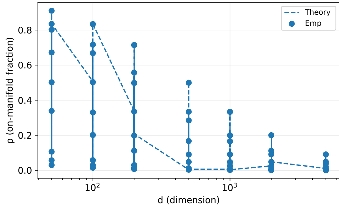
Exp 2c: \rho vs dimension d
