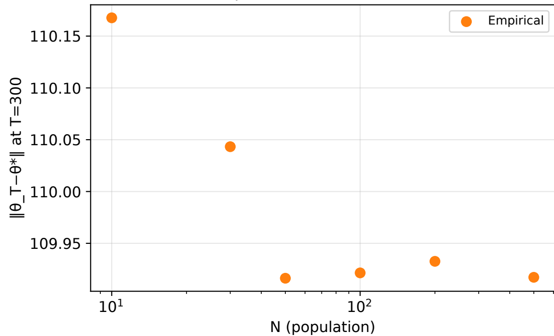
Exp 3e: Final distance vs N
