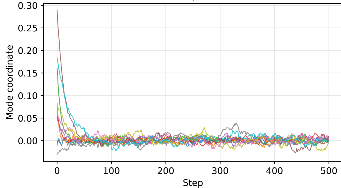
D1: Per-mode trajectories ( \sigma=0.5 )
