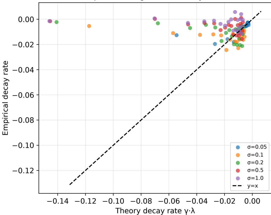
Exp D2: Per-eigenmode decay rates
