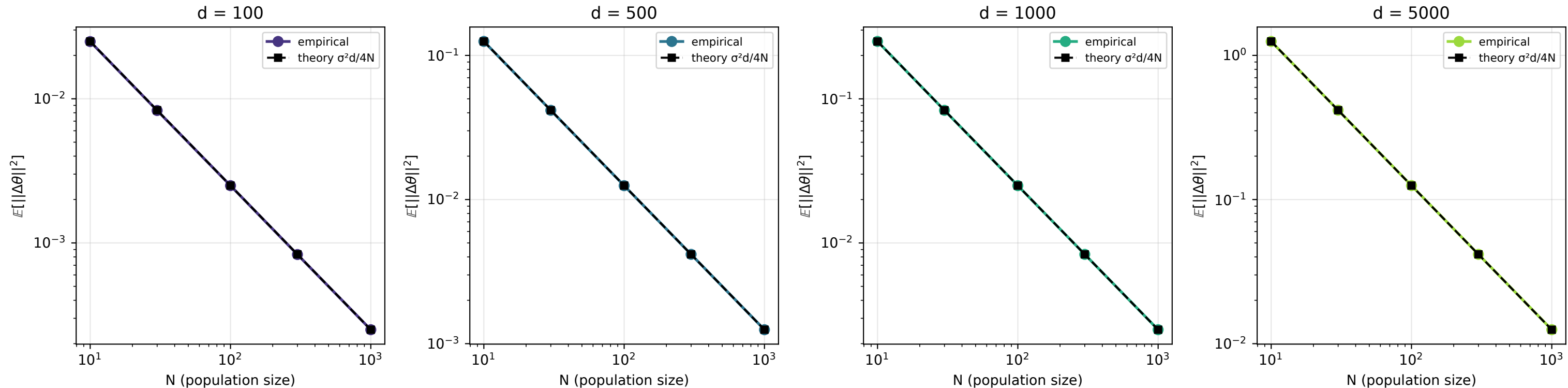
Exp 1a: One-step drift variance vs N (flat landscape)
