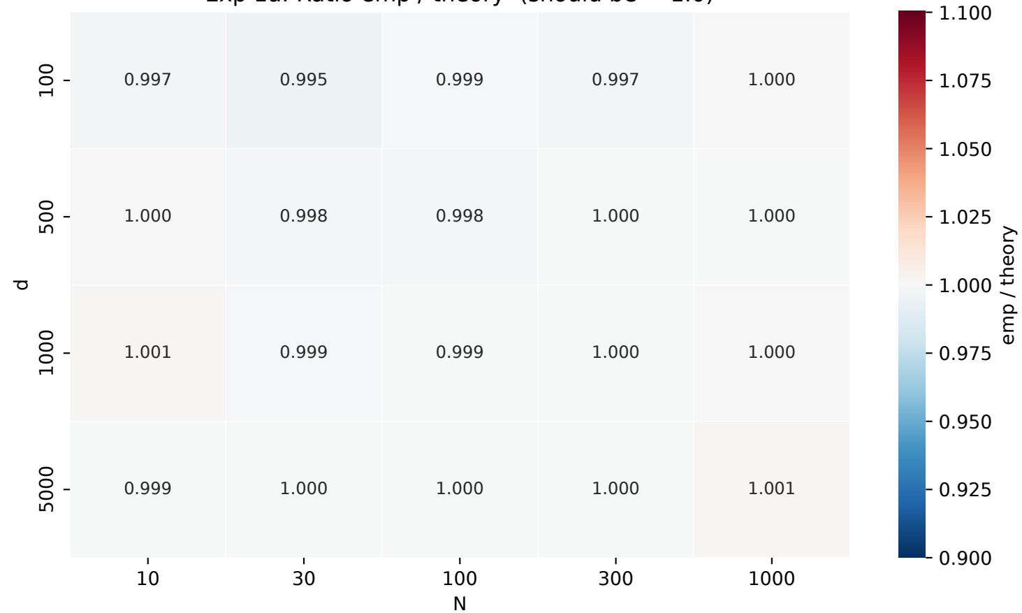
Exp 1a: Ratio emp / theory (should be \approx 1.0 )
