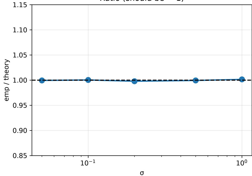
Ratio (should be \approx 1 )
