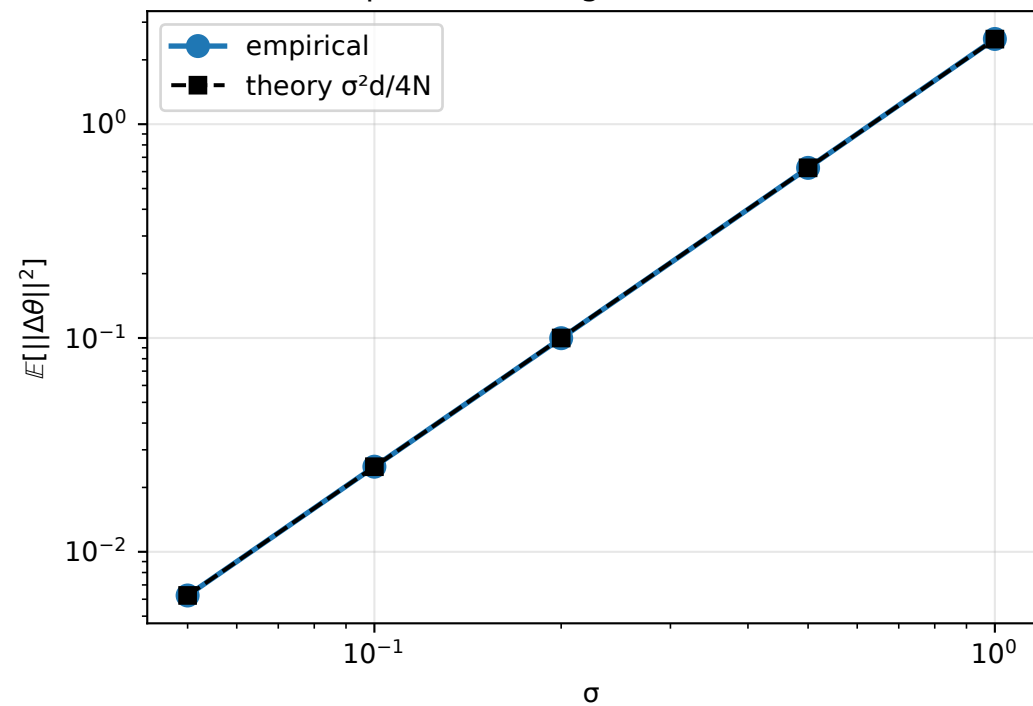
Exp 1b: \sigma scaling ( d=500 , N=50 )
