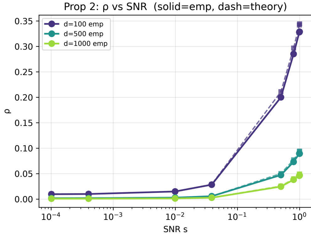
Exp 2a: On-manifold fraction \rho vs reward noise
