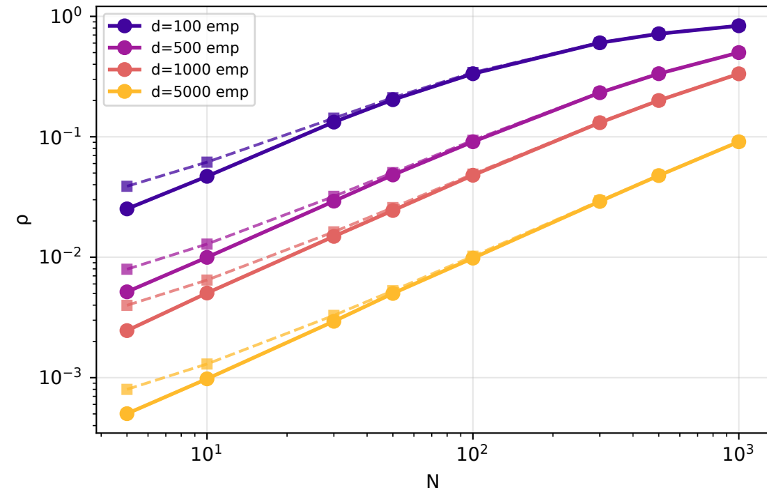
Exp 2b: \rho vs N ( \xi=0.1 , solid=emp, dash=theory)
