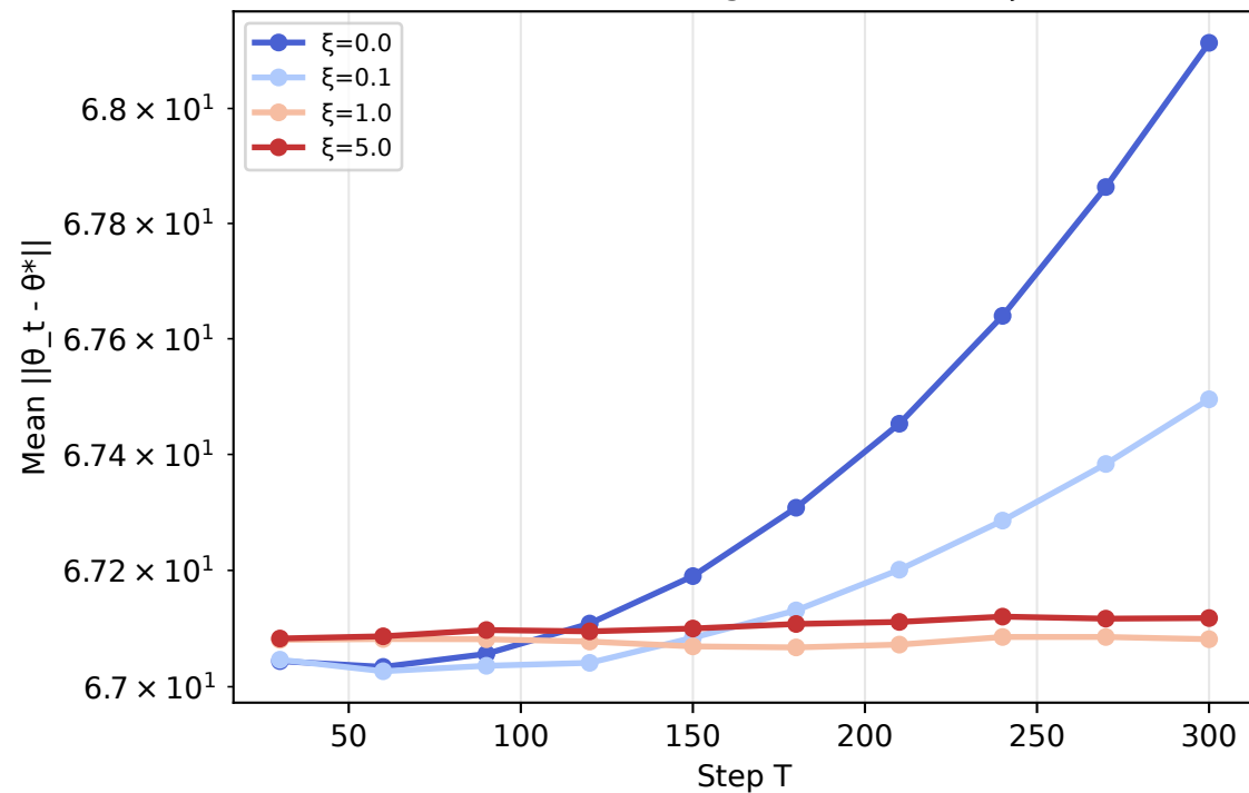
N=50: Convergence vs noise \xi
