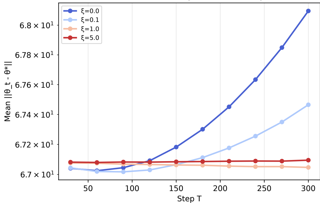
N=200: Convergence vs noise \xi
