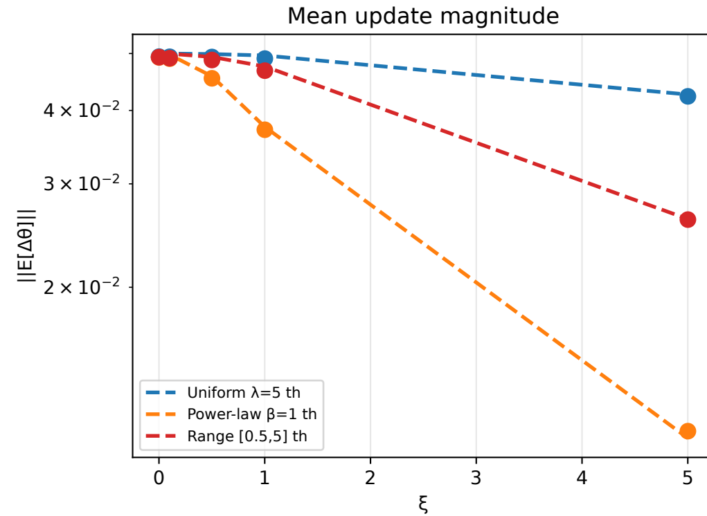
Exp 3a: \sigma_R and mean update — Prop 3 validation
