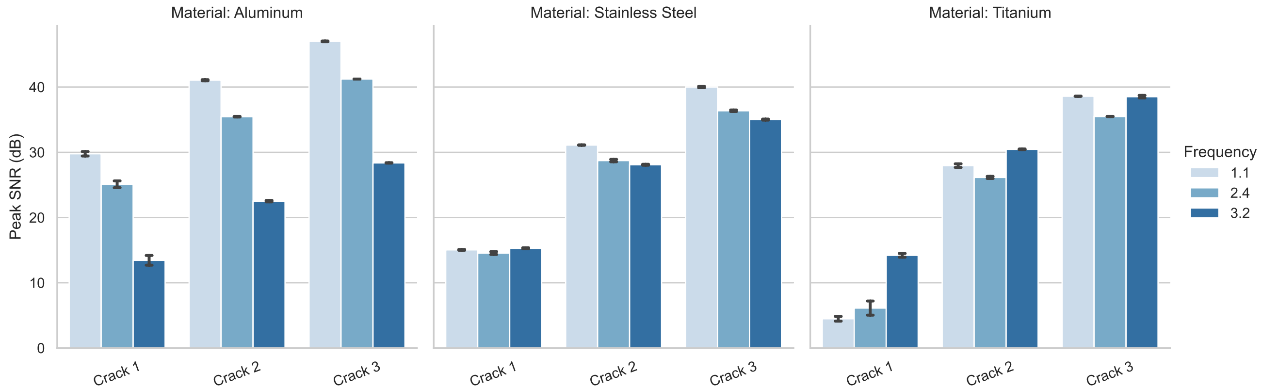
Peak SNR by Crack Size and Frequency (Faceted by Material)
