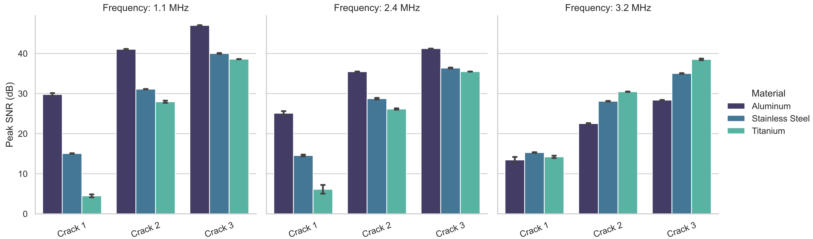
Peak SNR by Crack Size and Material (Faceted by Frequency)
