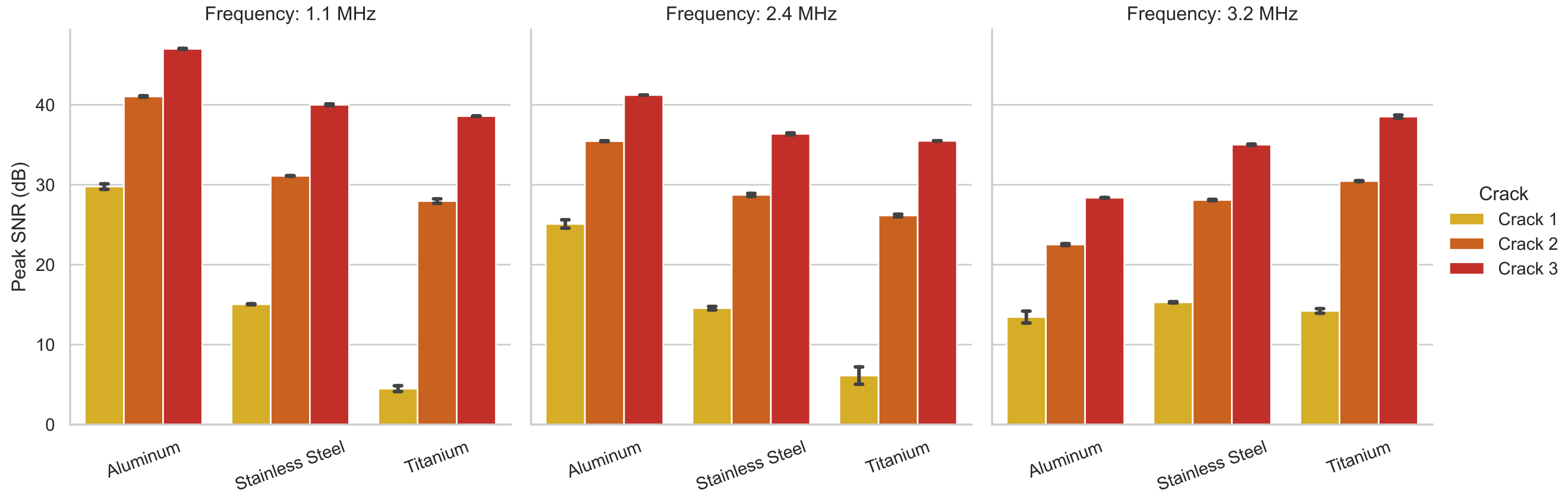
Peak SNR by Material, Crack, and Frequency
