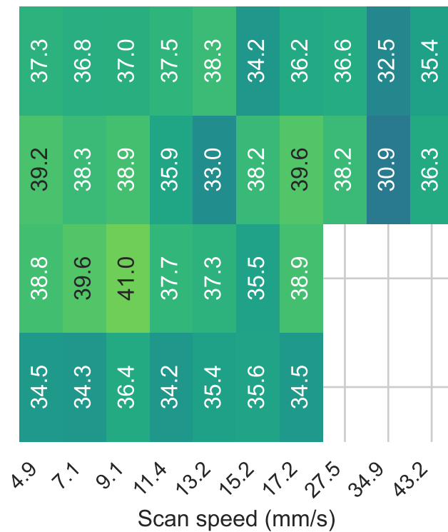
0.020" notch
