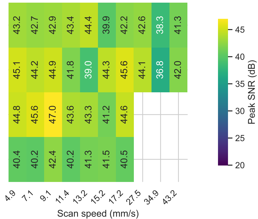
0.040" notch
