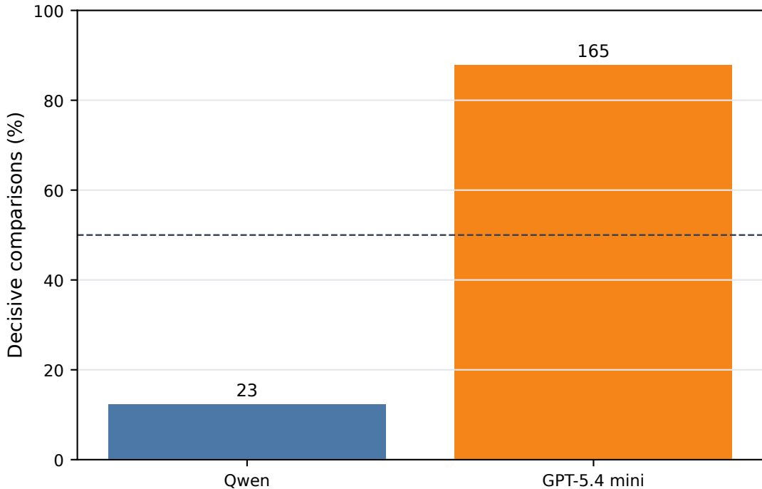
Decisive Pairwise Win Share
