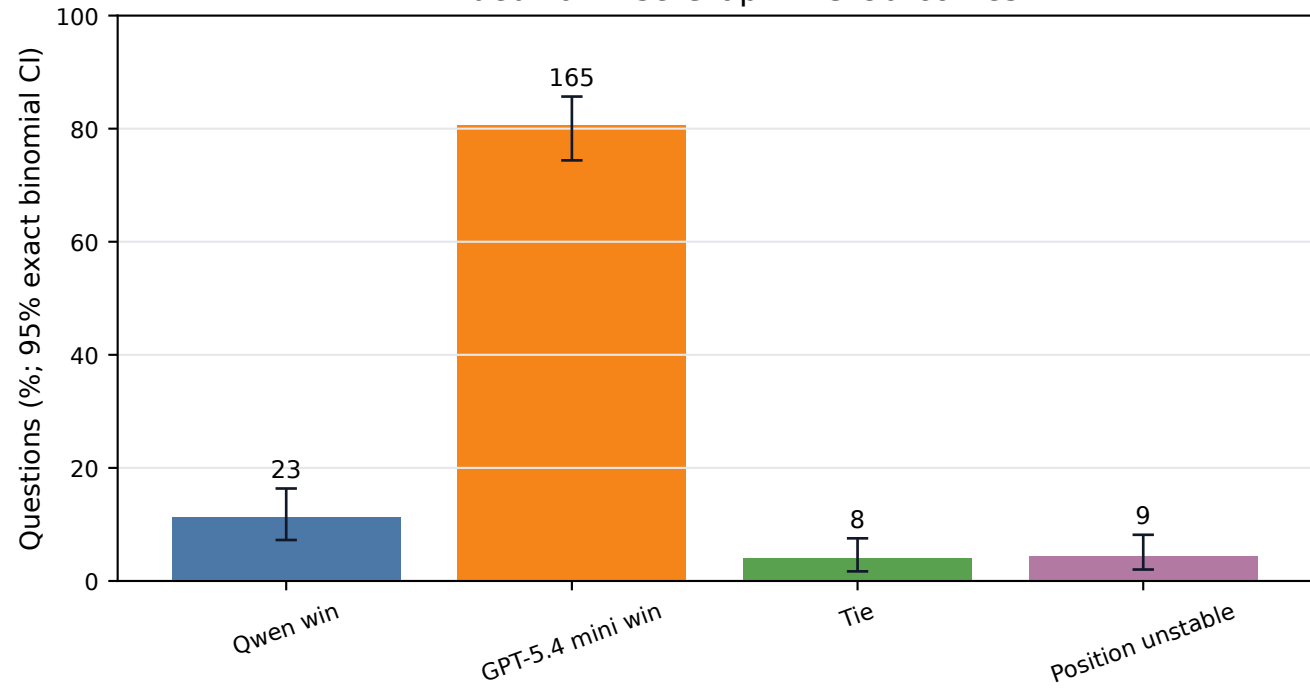
Blinded Pairwise GraphRAG Outcomes
