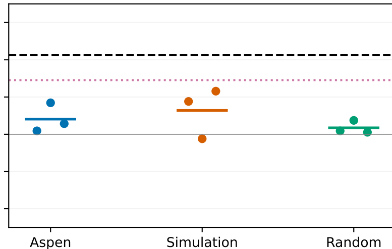
Three-prong; common-pT
