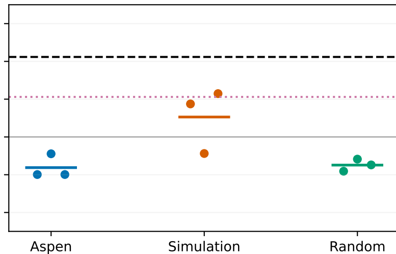
Three-prong; common-pT
