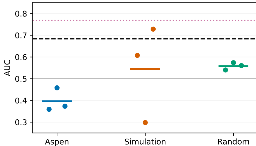
Three-prong; original
