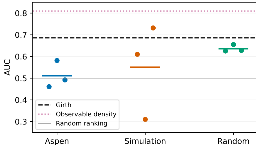
Three-prong; original
