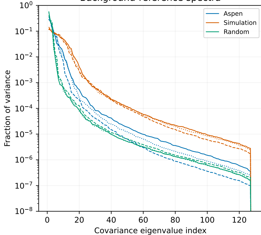
Background-reference spectra
