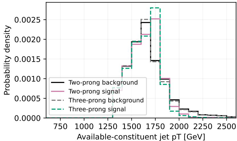
Common-pT weighted population
