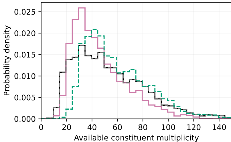
Common-pT weighted population
