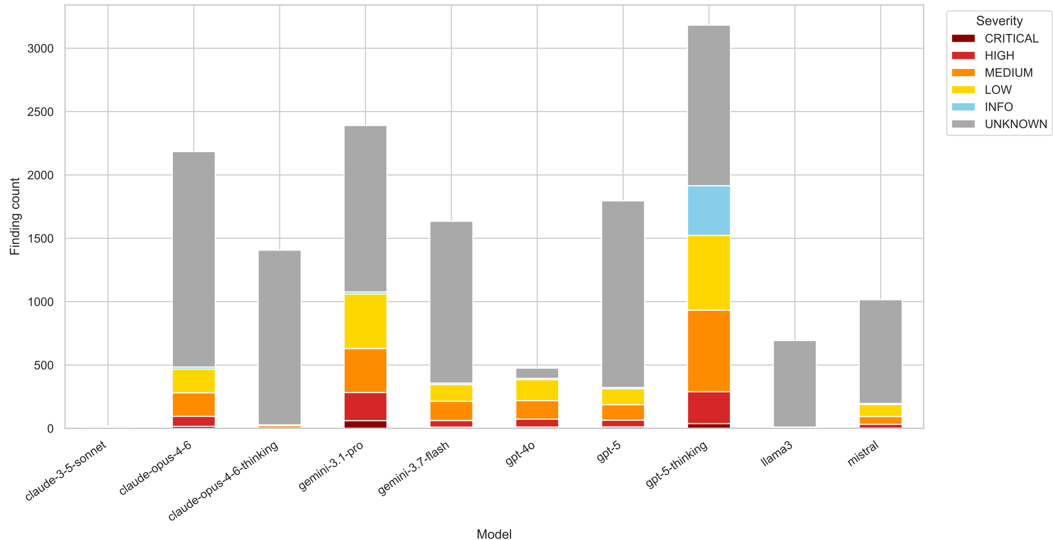
Severity Distribution of Findings by Model
