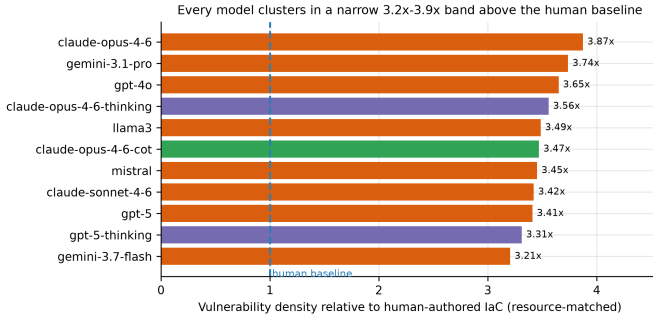
Fig. 4. Per-configuration density relative to the human baseline. Purple: vendor extended thinking. Green: prompted chain-of-thought.
