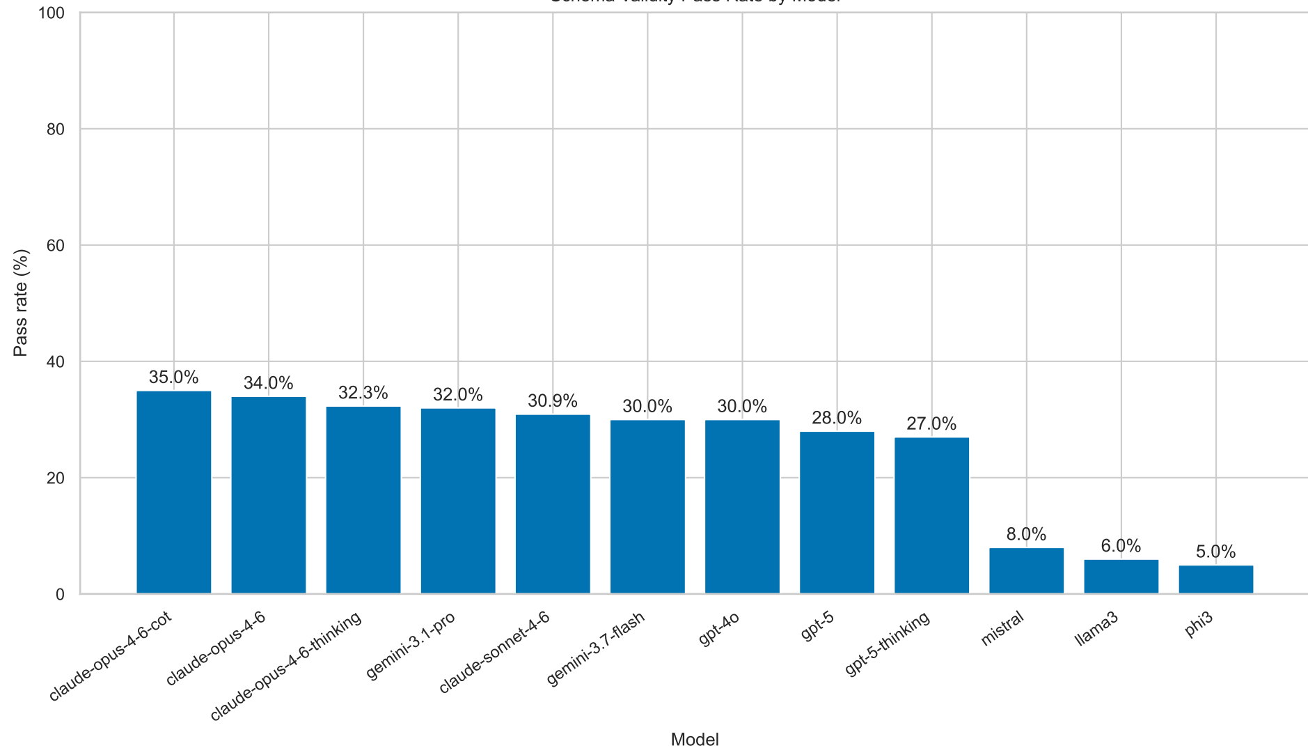
Schema Validity Pass Rate by Model
