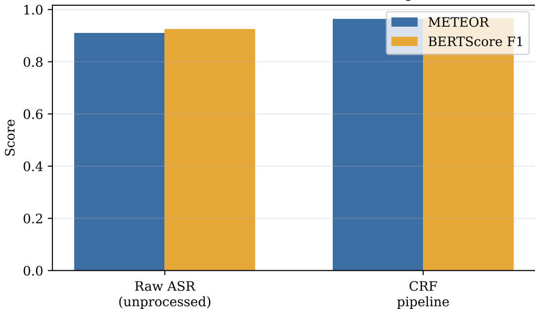
METEOR and BERTScore (test split)
