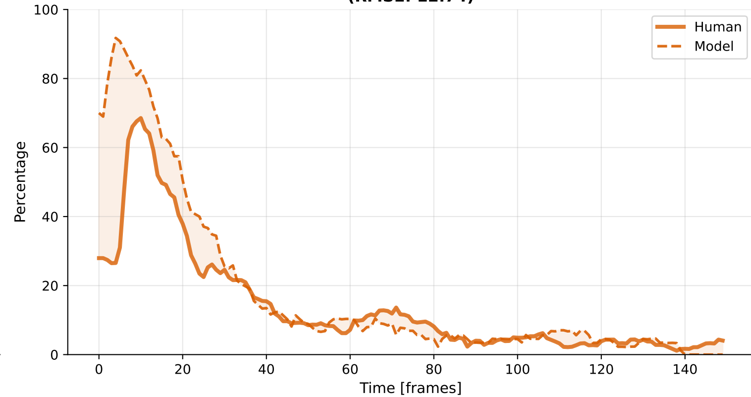
Revisit (RMSE: 26.69)
