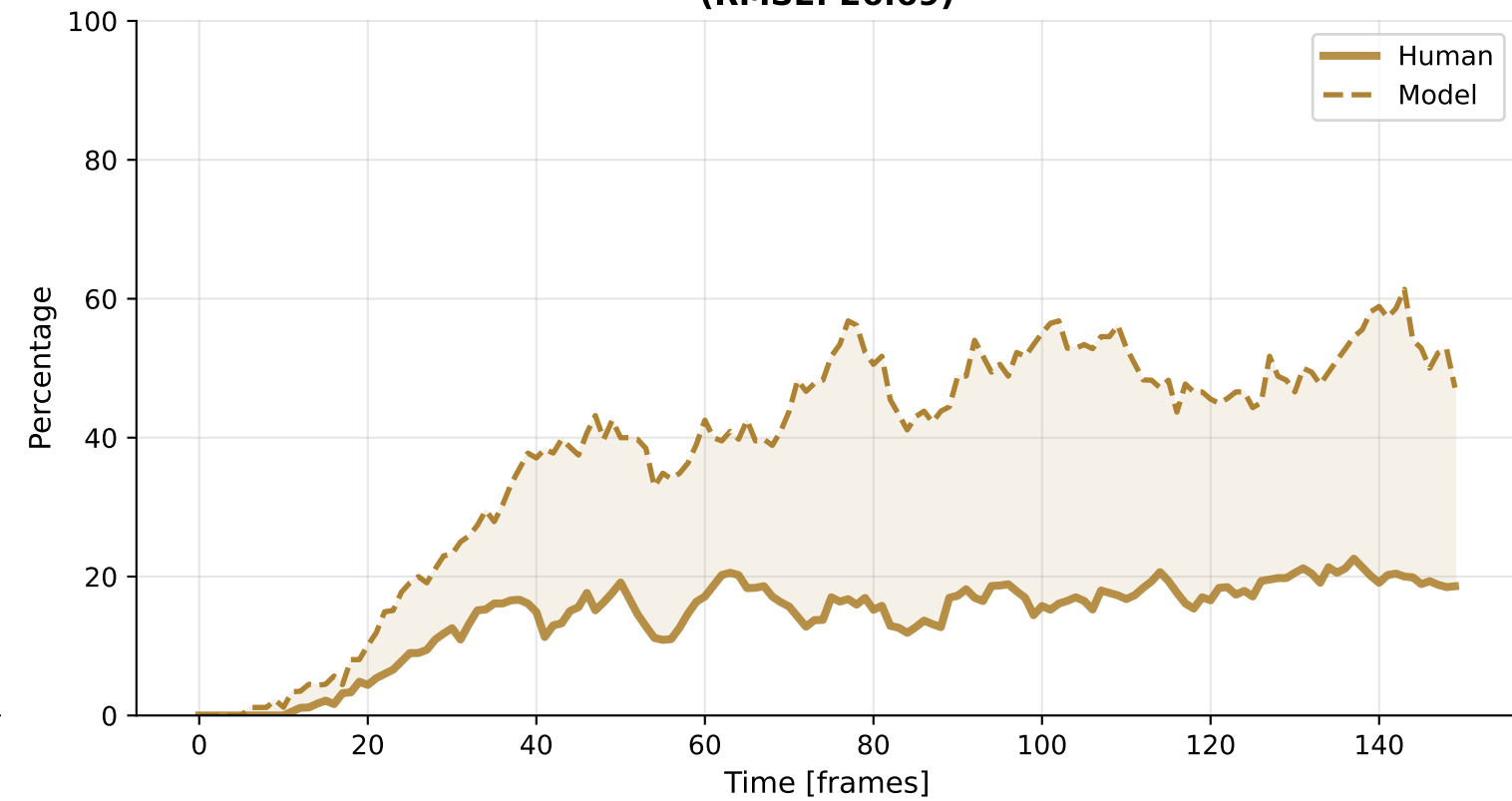
Revisit (RMSE: 26.69)
