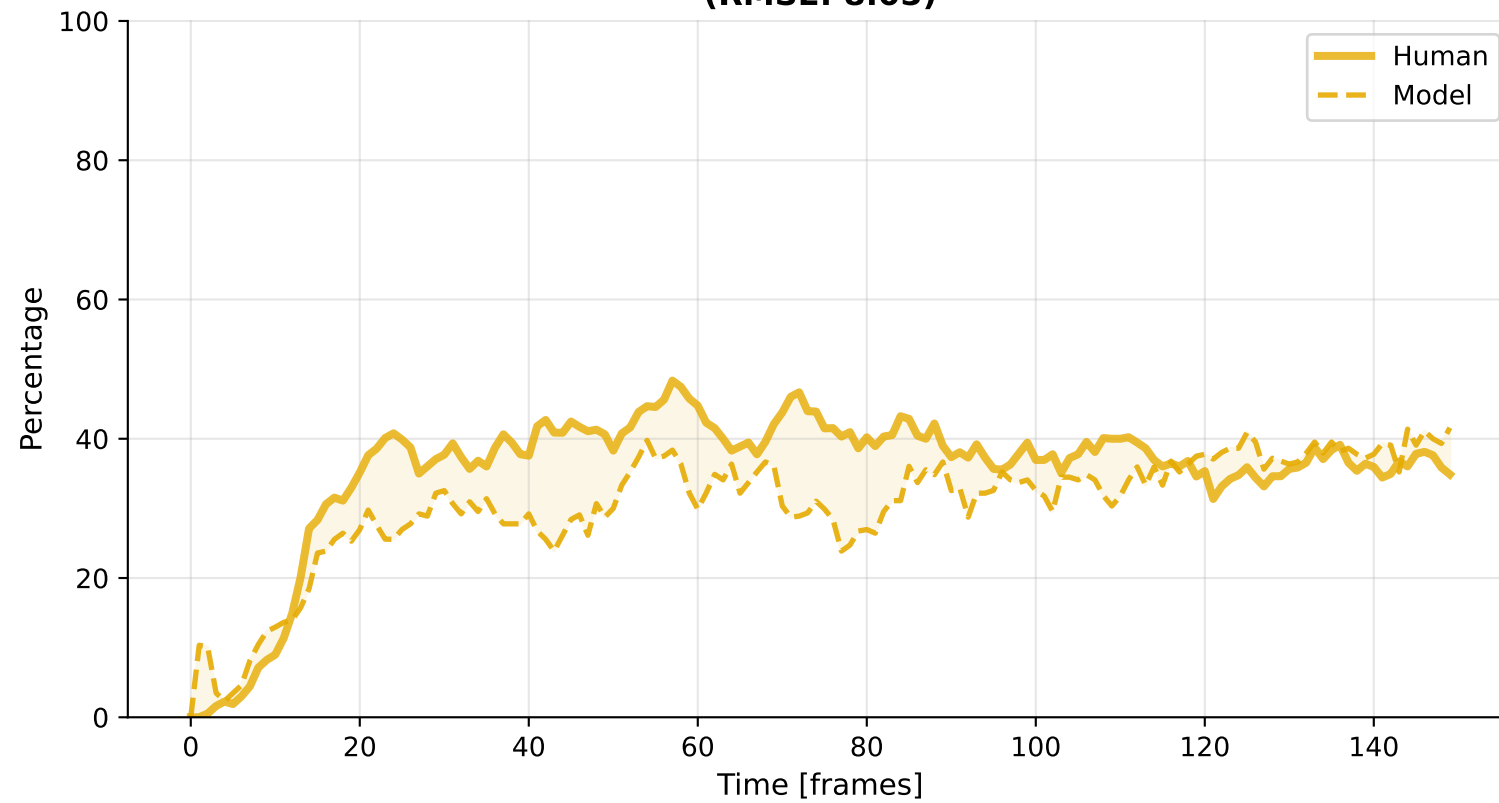
Inspection (RMSE: 8.05)
