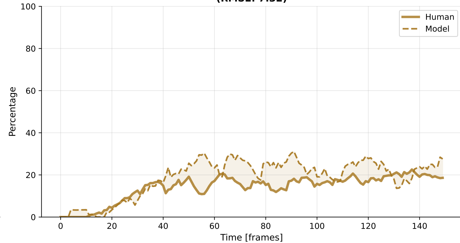
Revisit (RMSE: 7.32)
