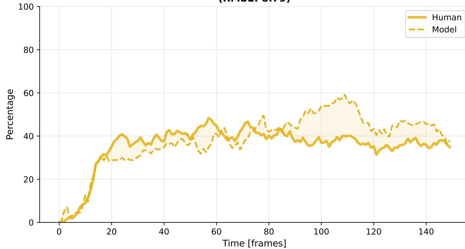
Inspection (RMSE: 8.79)
