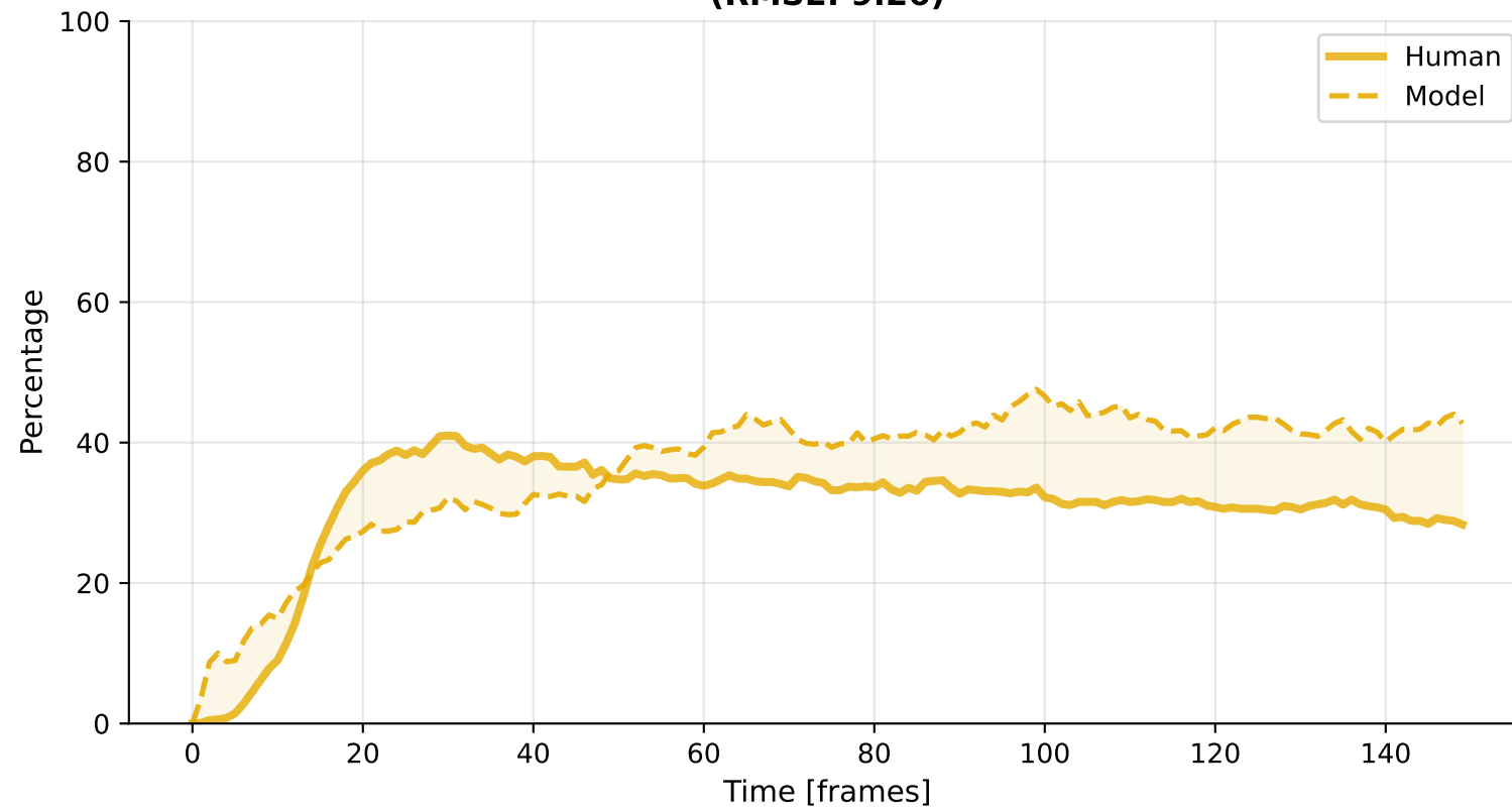
Inspection (RMSE: 9.26)
