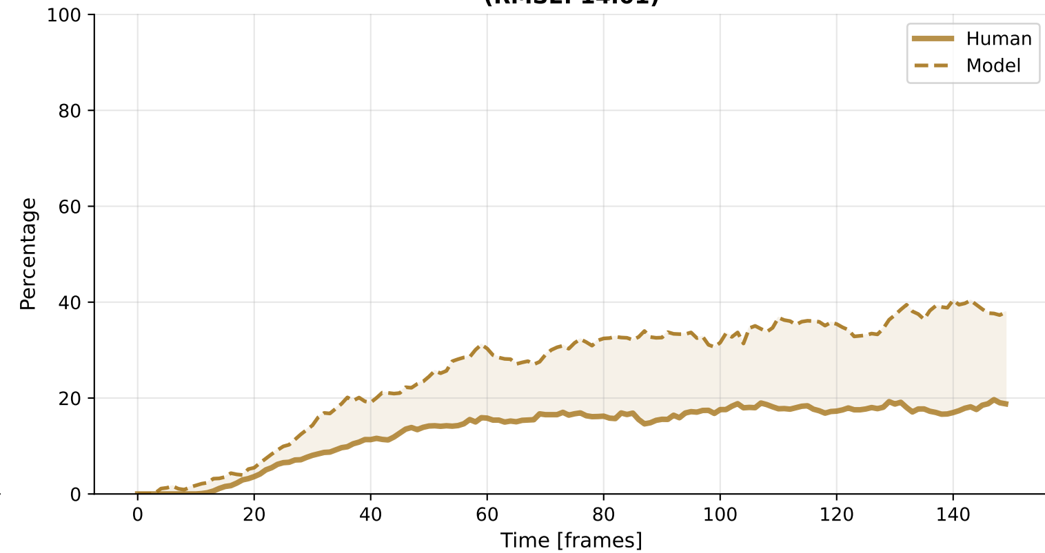
Revisit (RMSE: 14.01)
