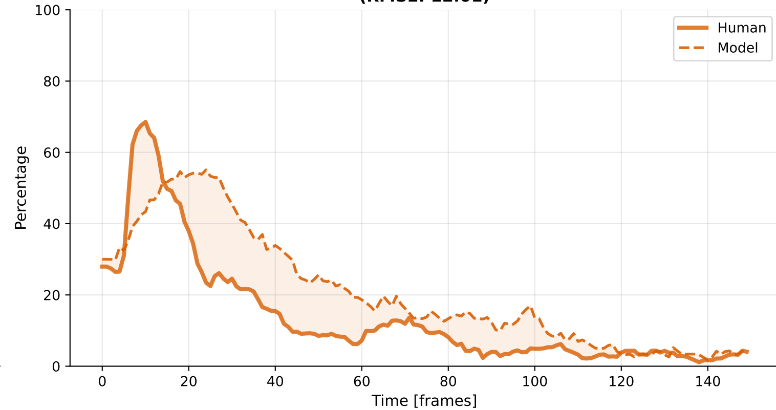
Revisit (RMSE: 8.72)
