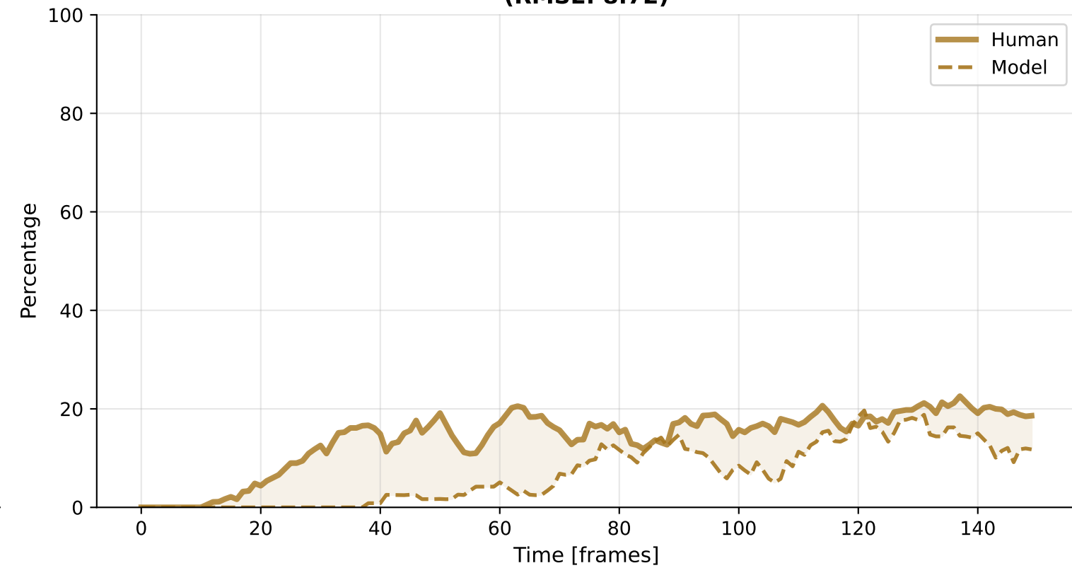
Revisit (RMSE: 8.72)
