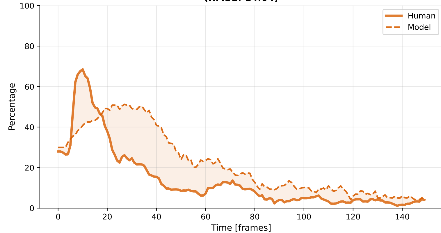
Revisit (RMSE: 10.02)
