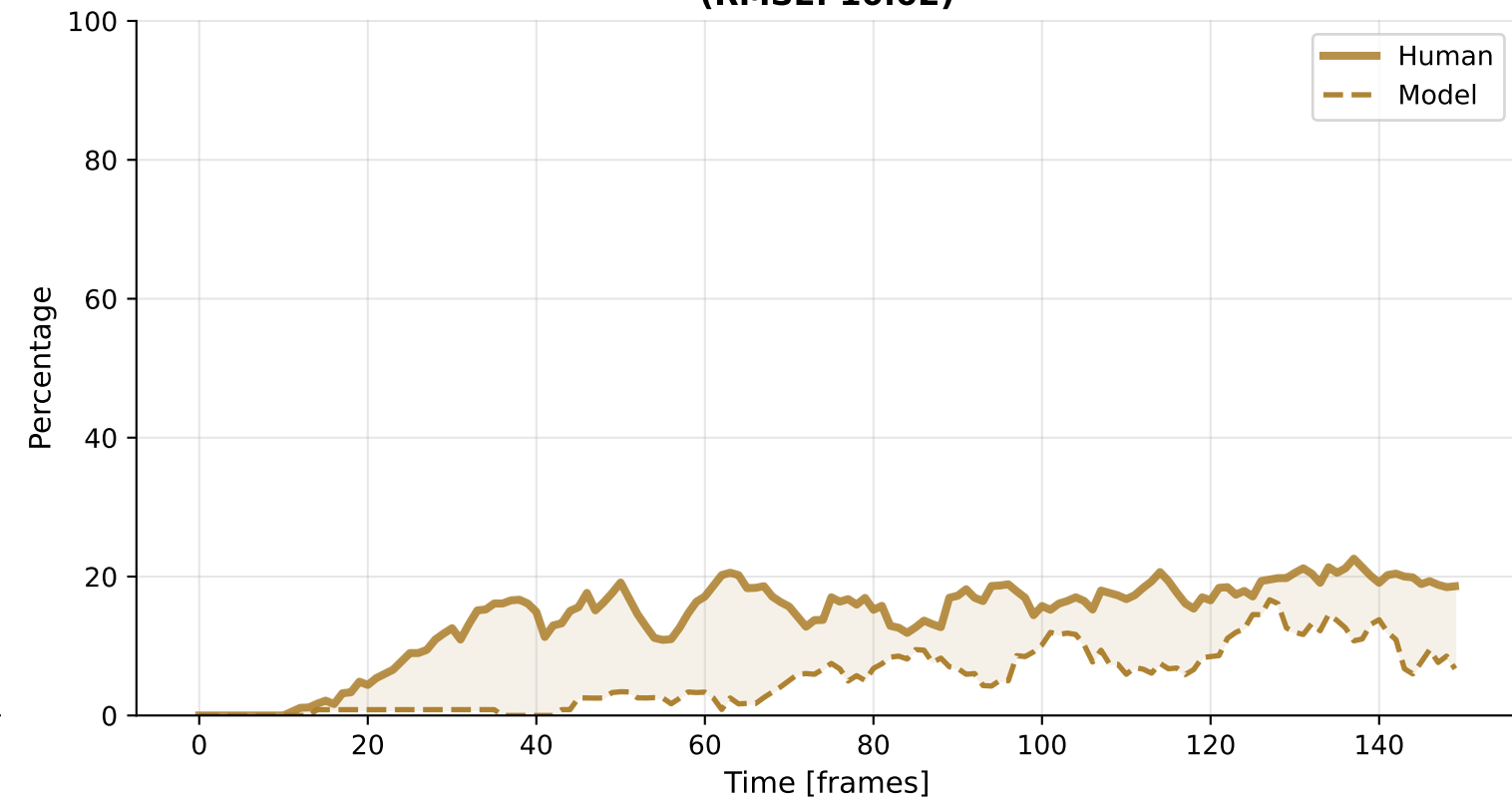
Revisit (RMSE: 10.02)
