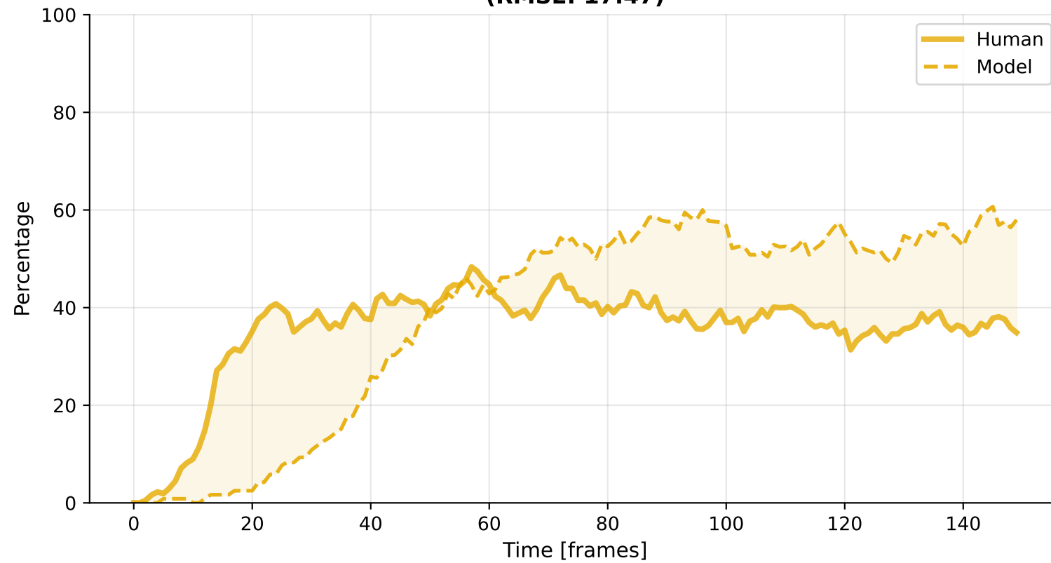
Inspection (RMSE: 17.47)
