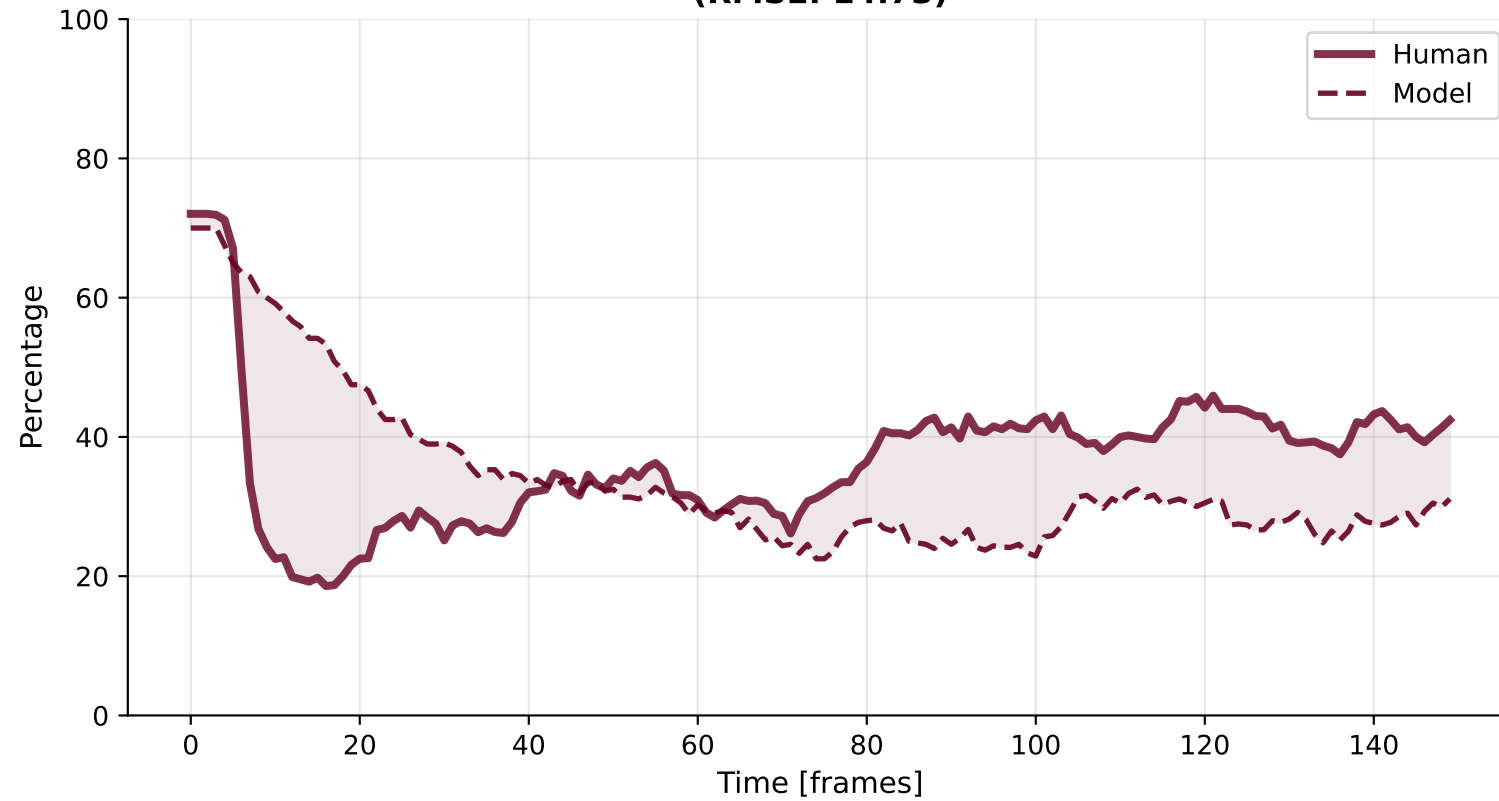
Inspection (RMSE: 17.47)
