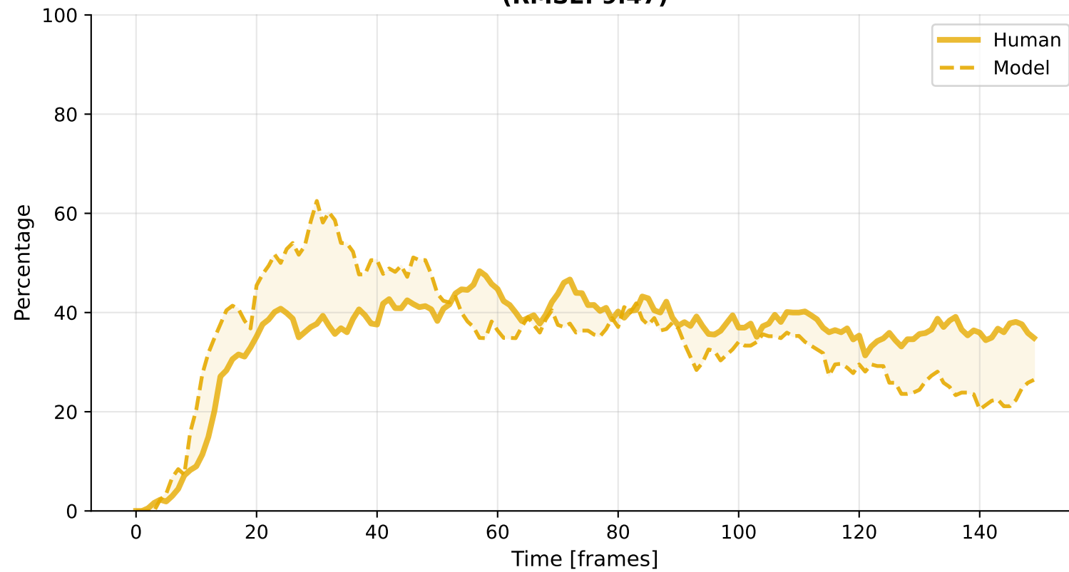
Inspection (RMSE: 9.47)
