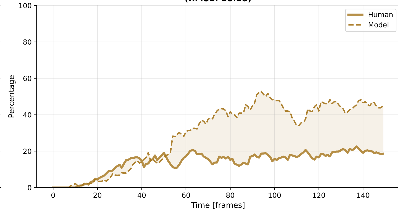
Revisit (RMSE: 20.25)
