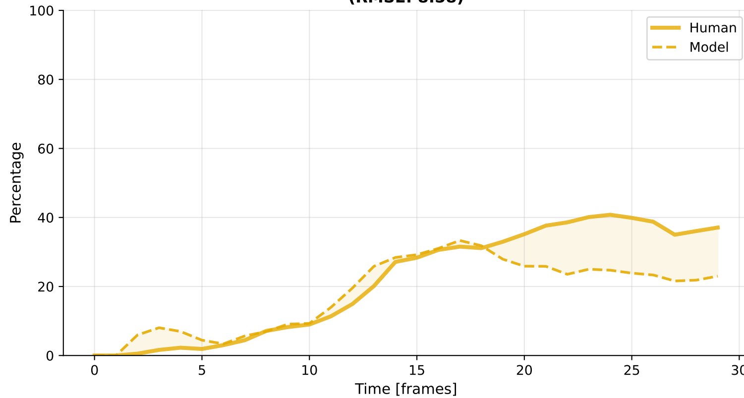
Inspection (RMSE: 8.58)
