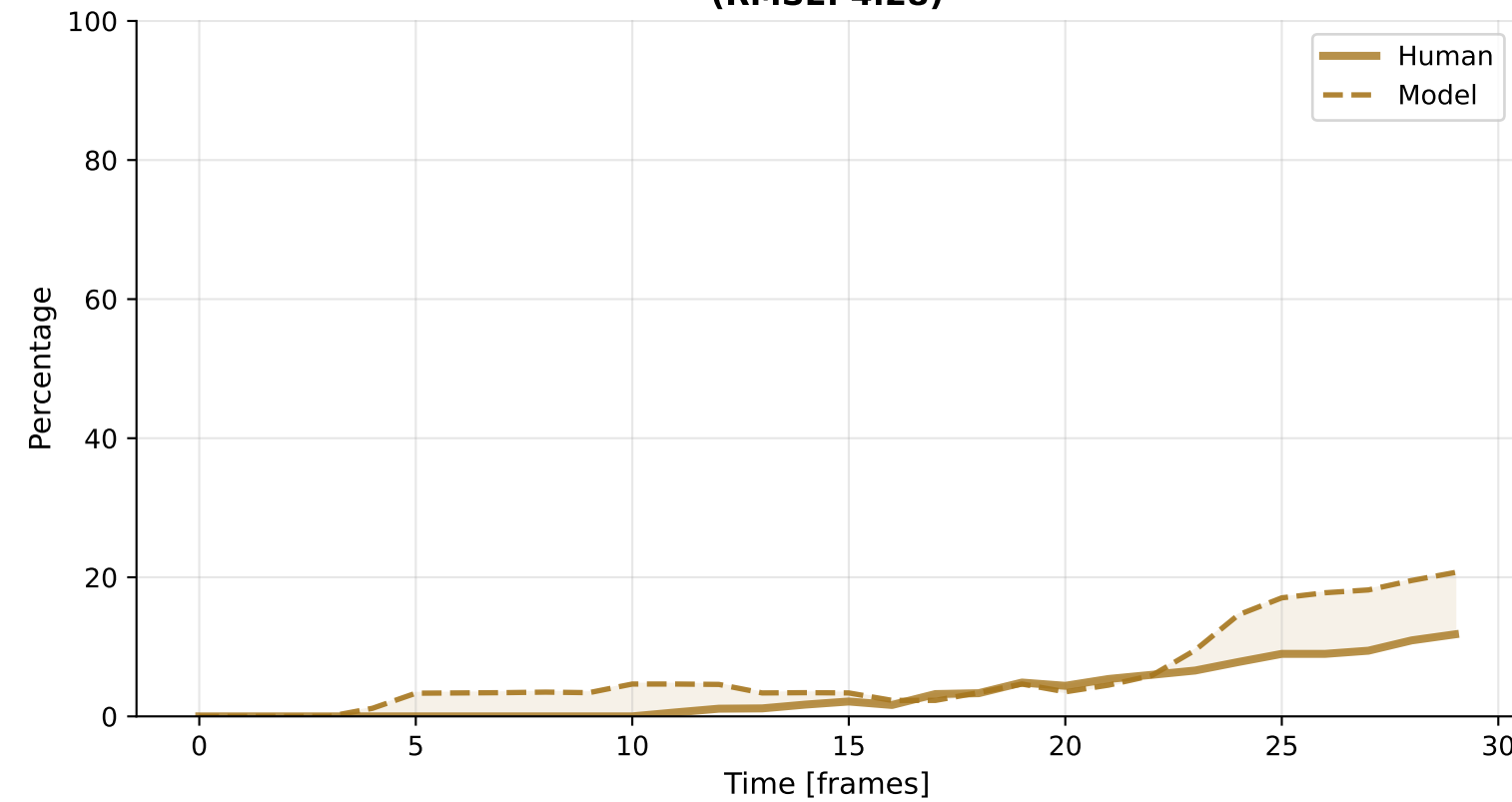
Revisit (RMSE: 4.28)
