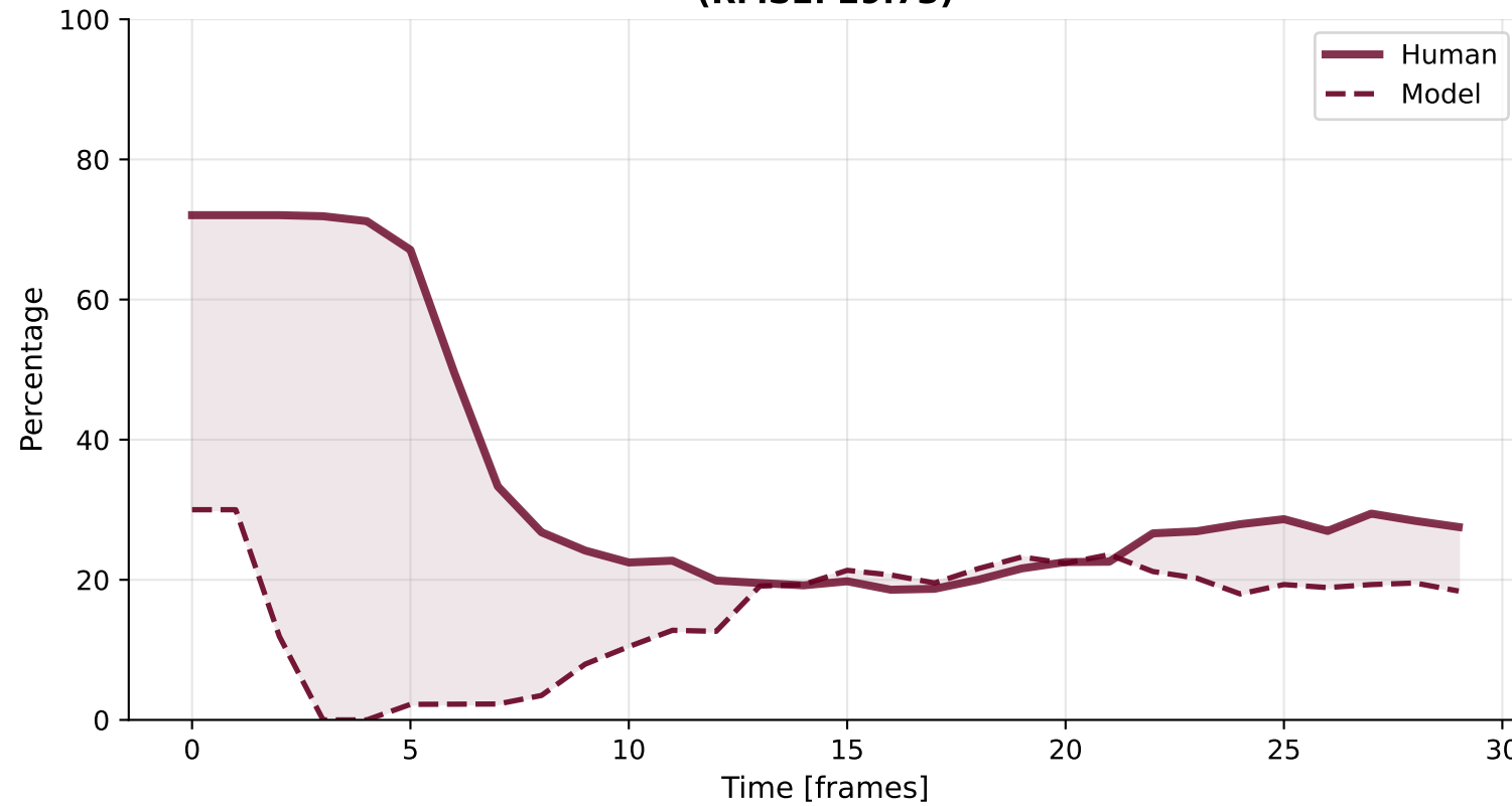
Inspection (RMSE: 8.58)
