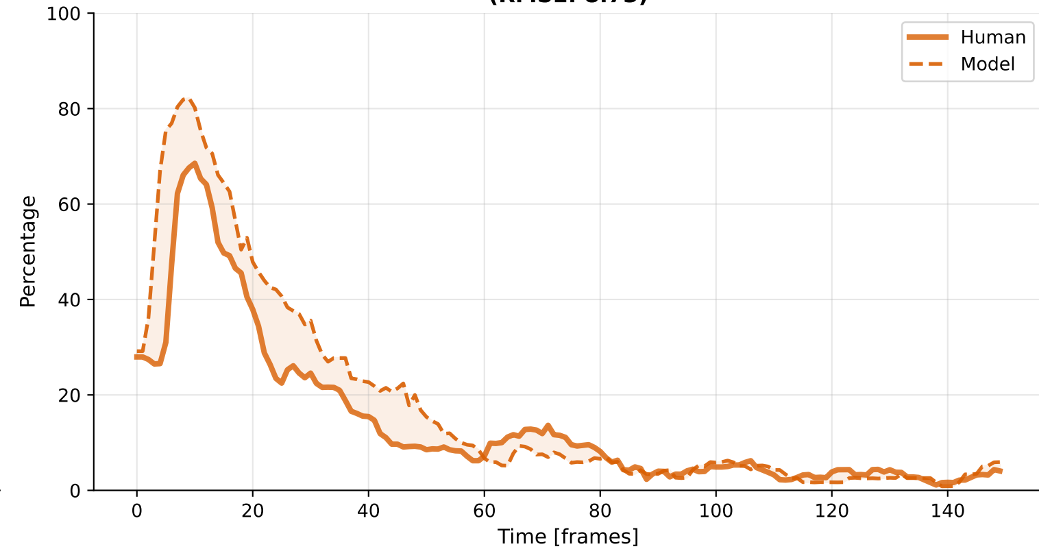
Revisit (RMSE: 5.76)
