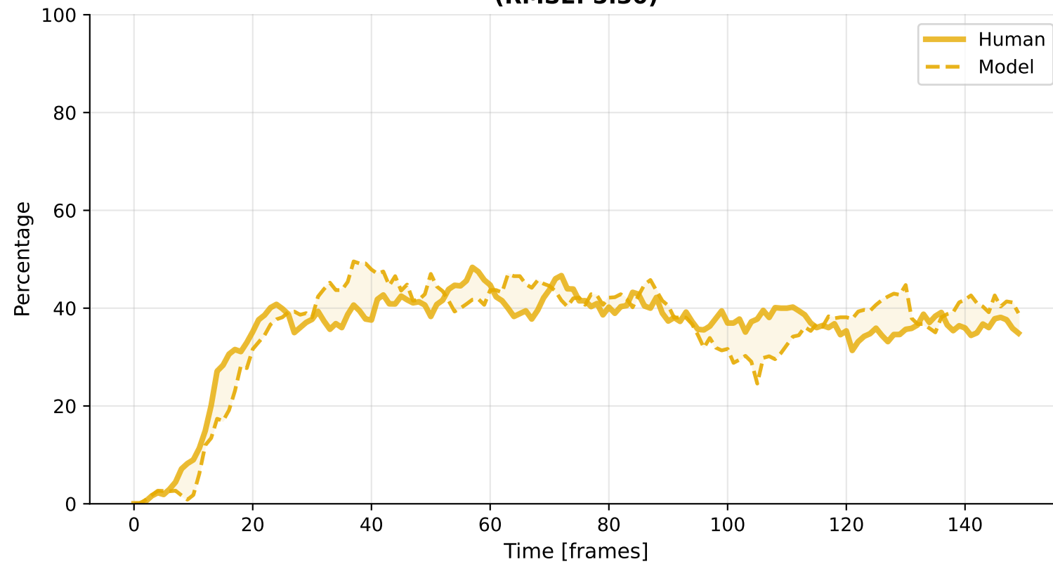
Inspection (RMSE: 5.30)
