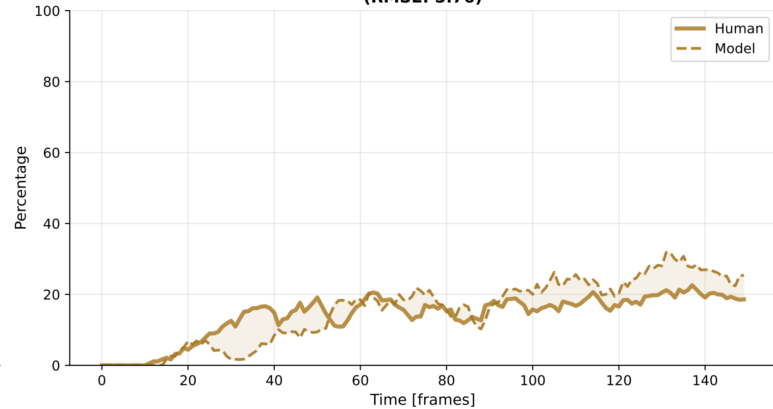
Revisit (RMSE: 5.76)
