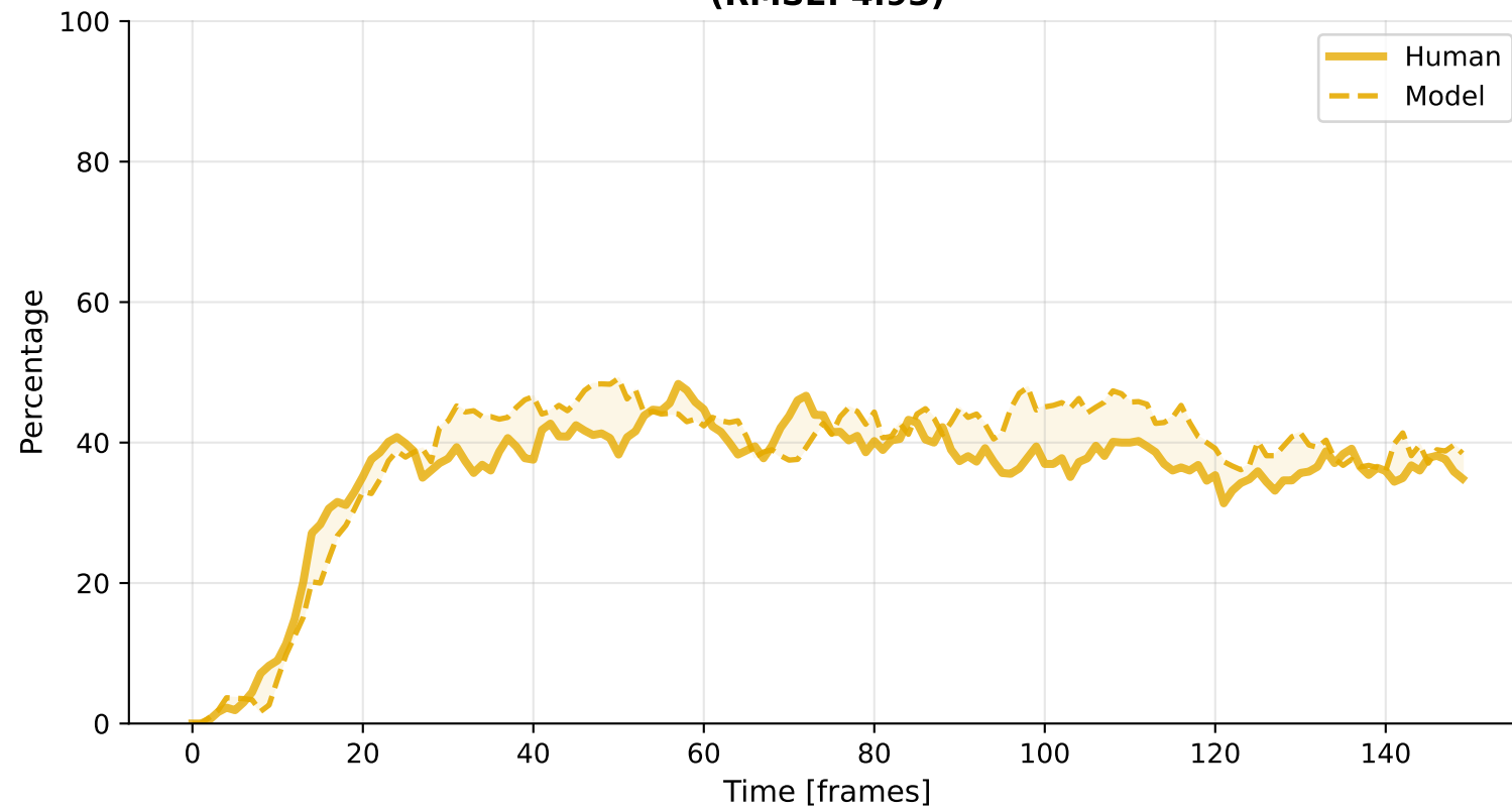
Inspection (RMSE: 4.93)
