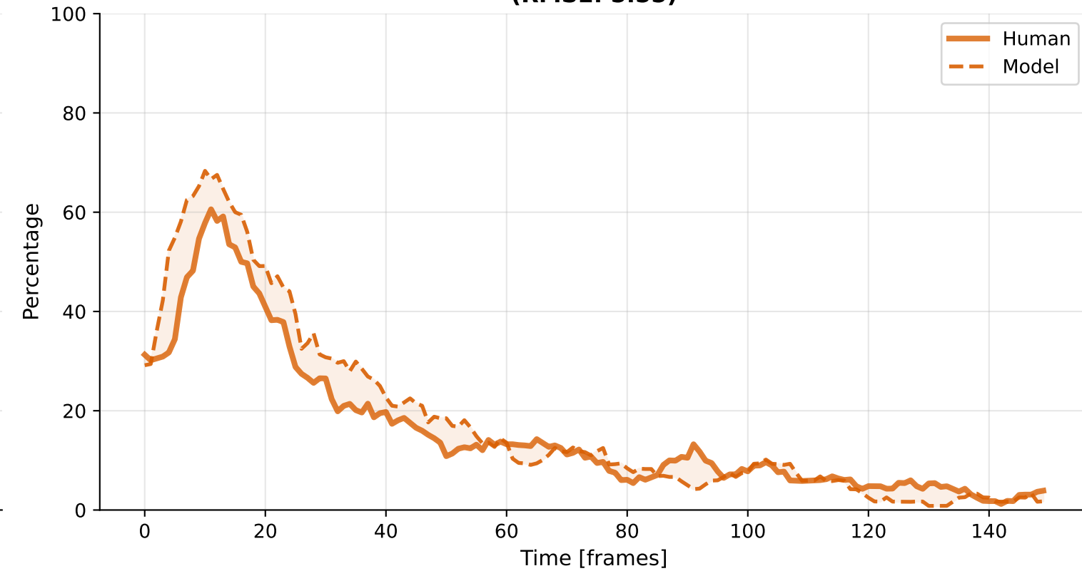
Revisit (RMSE: 5.85)
