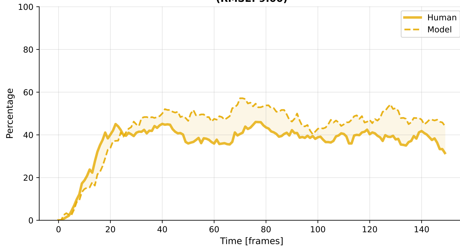
Inspection (RMSE: 9.00)
