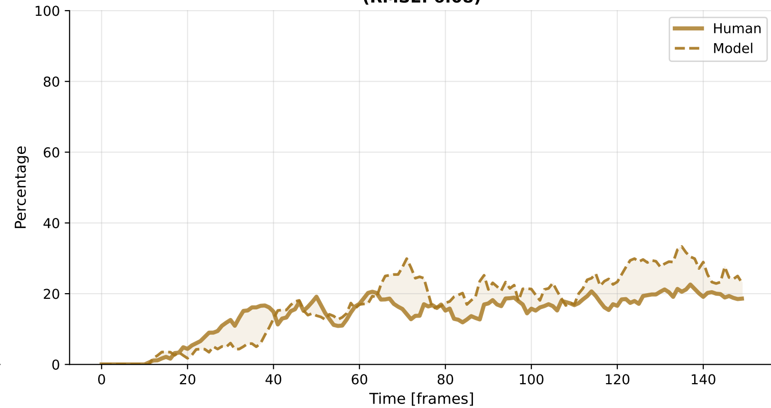
Revisit (RMSE: 6.08)
