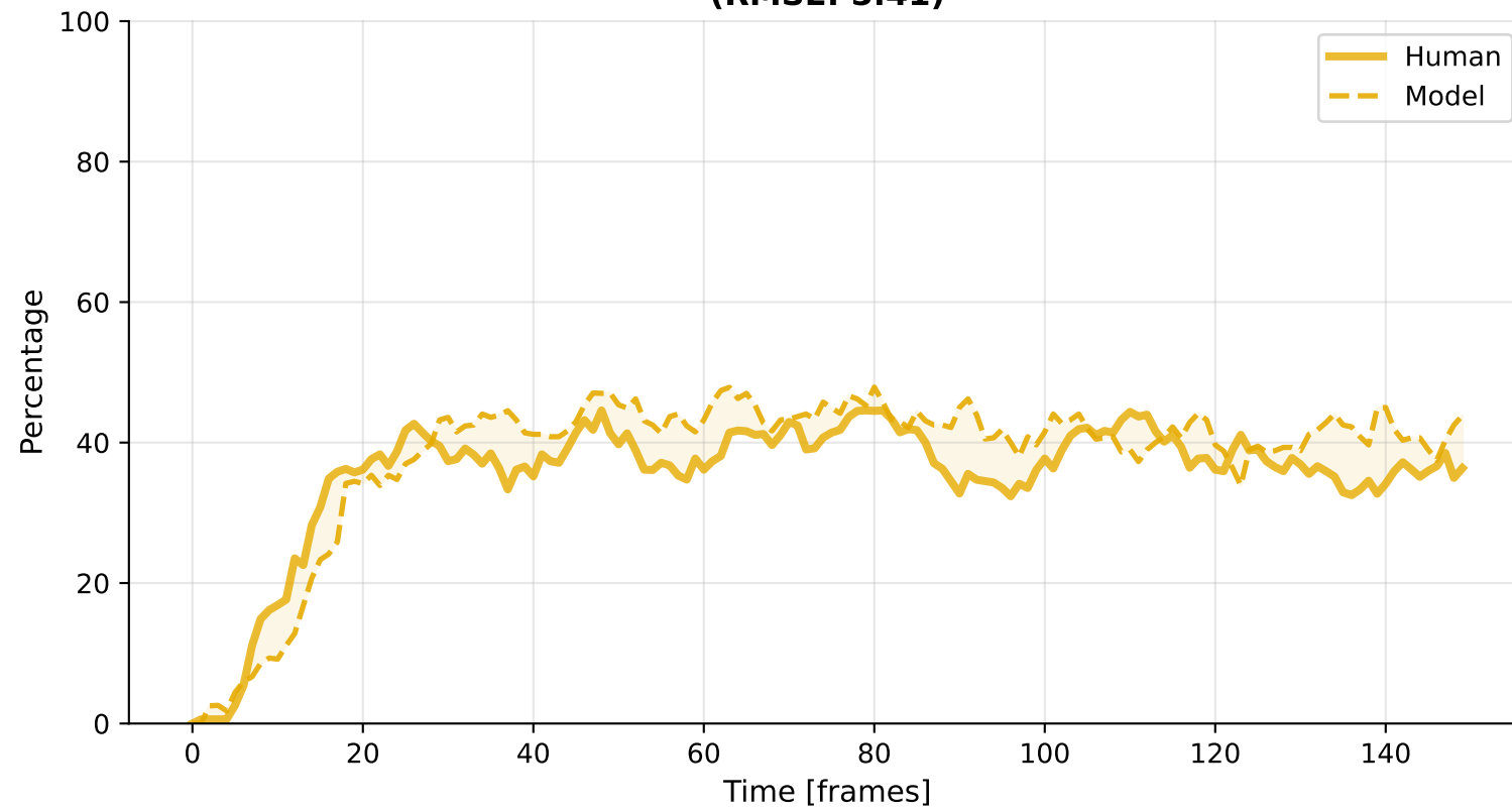
Inspection (RMSE: 5.41)
