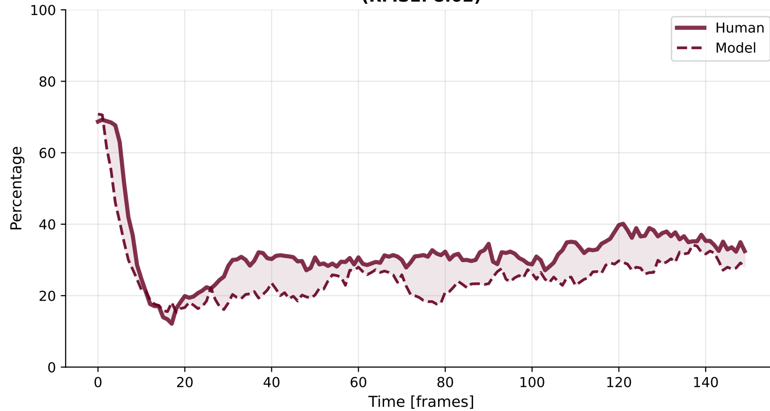
Inspection (RMSE: 5.41)
