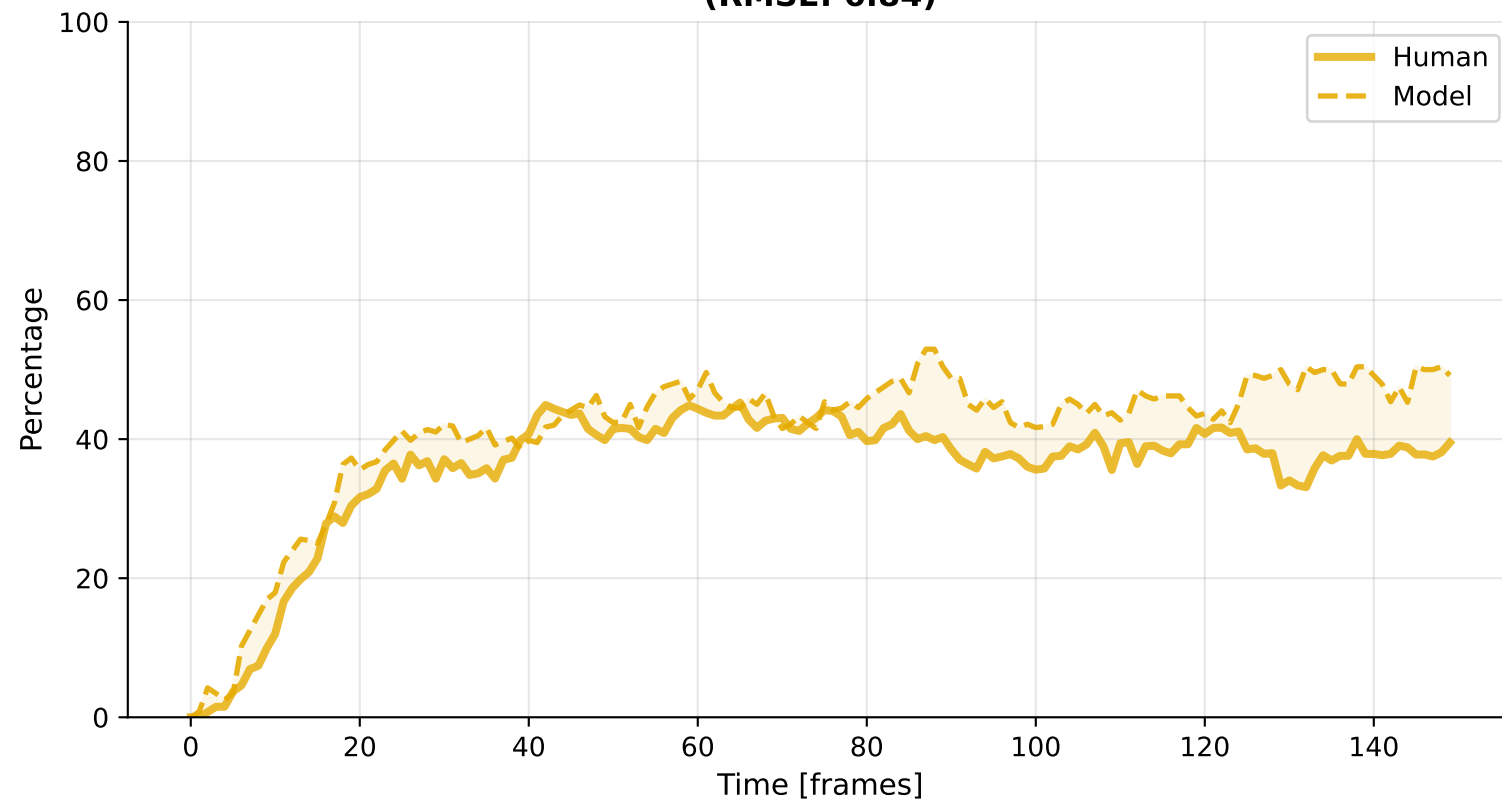
Inspection (RMSE: 6.84)
