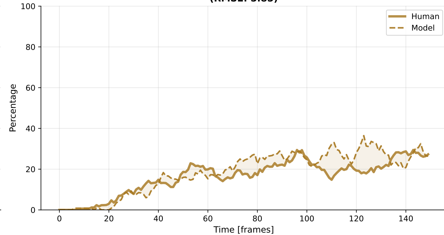
Revisit (RMSE: 5.85)
