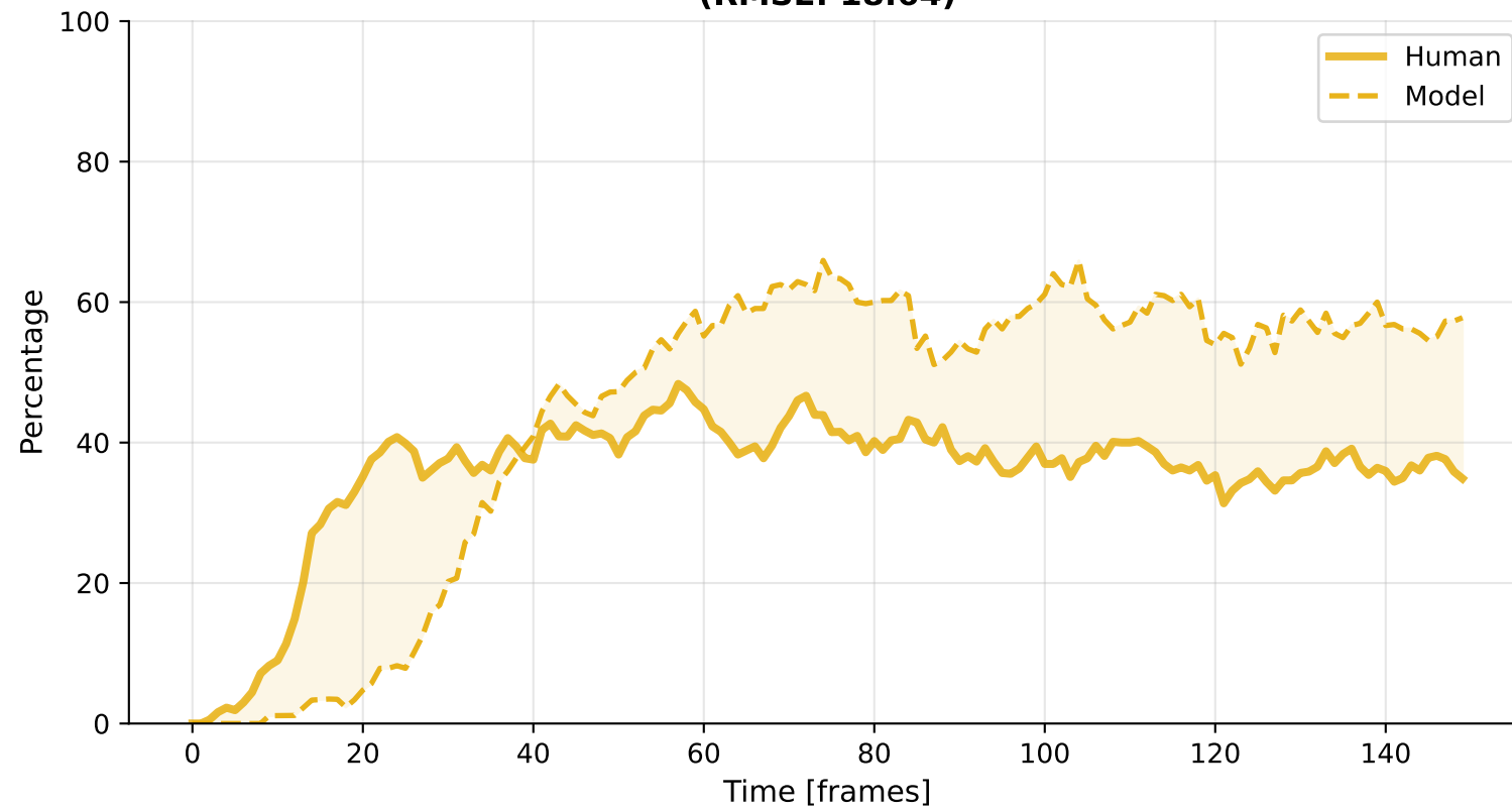
Inspection (RMSE: 18.64)
