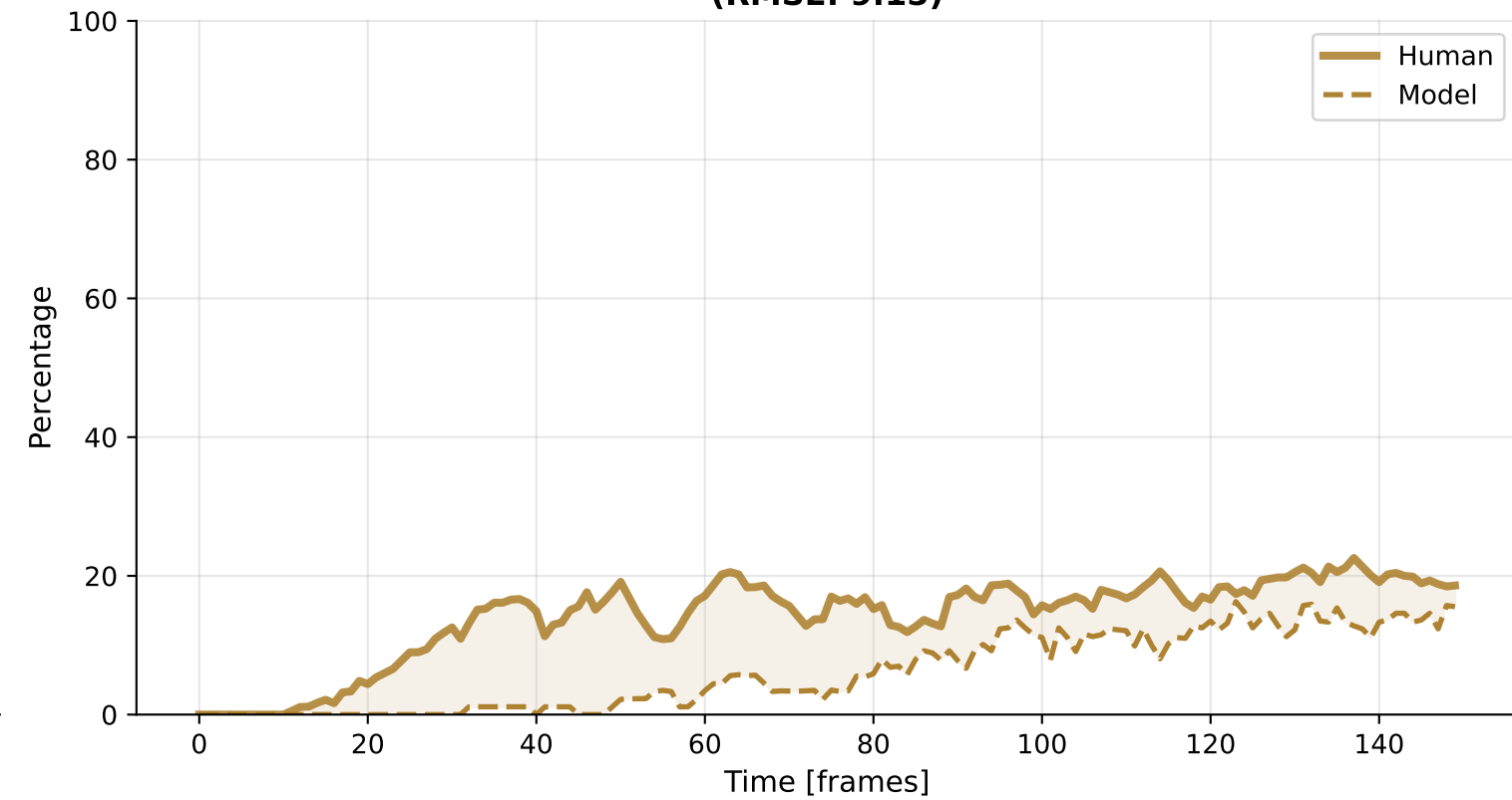
Revisit (RMSE: 9.15)
