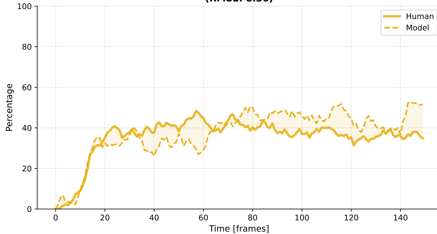
Inspection (RMSE: 8.36)
