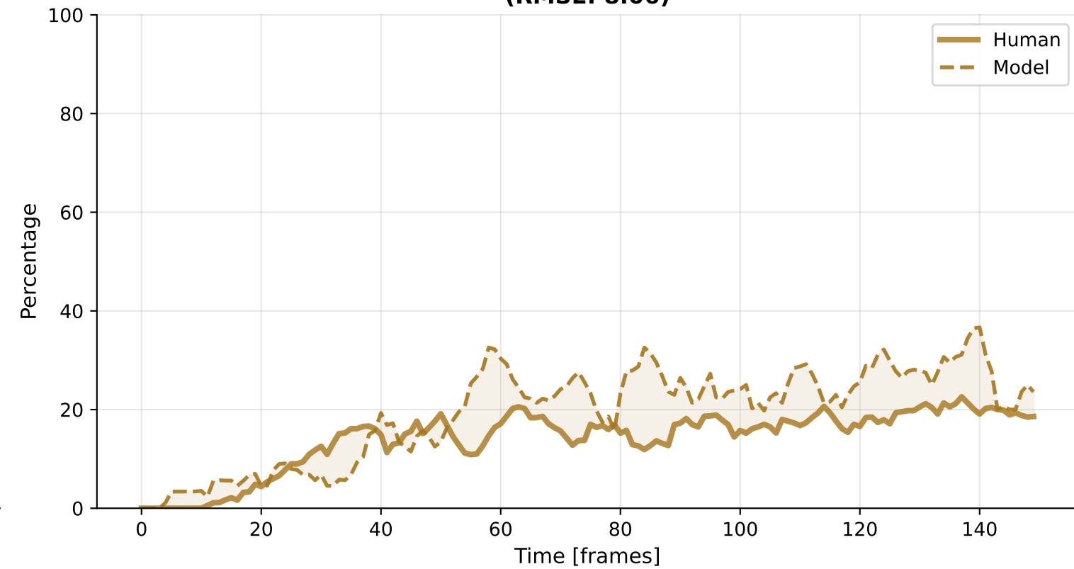
Revisit (RMSE: 8.06)
