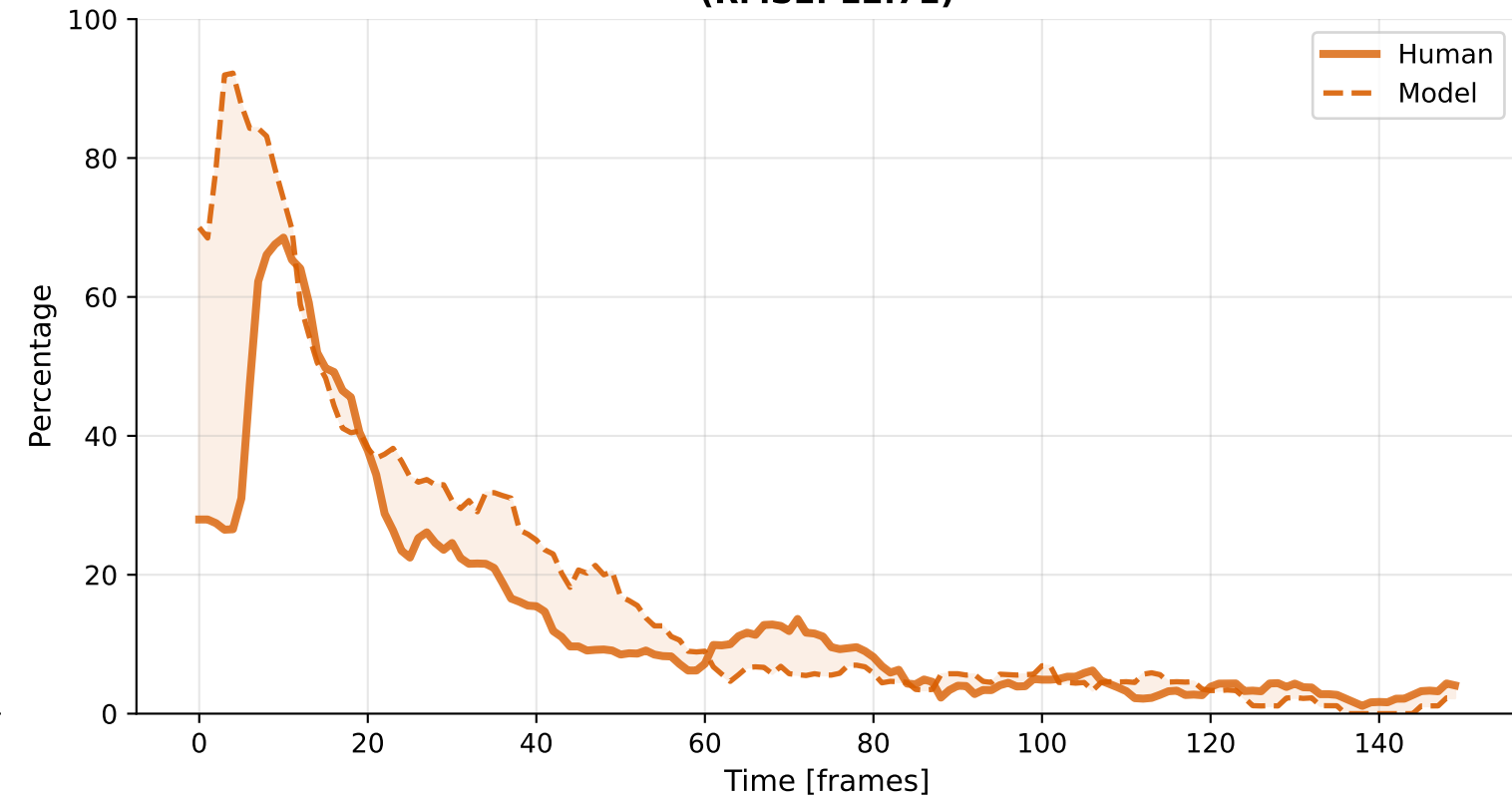
Revisit (RMSE: 8.06)
