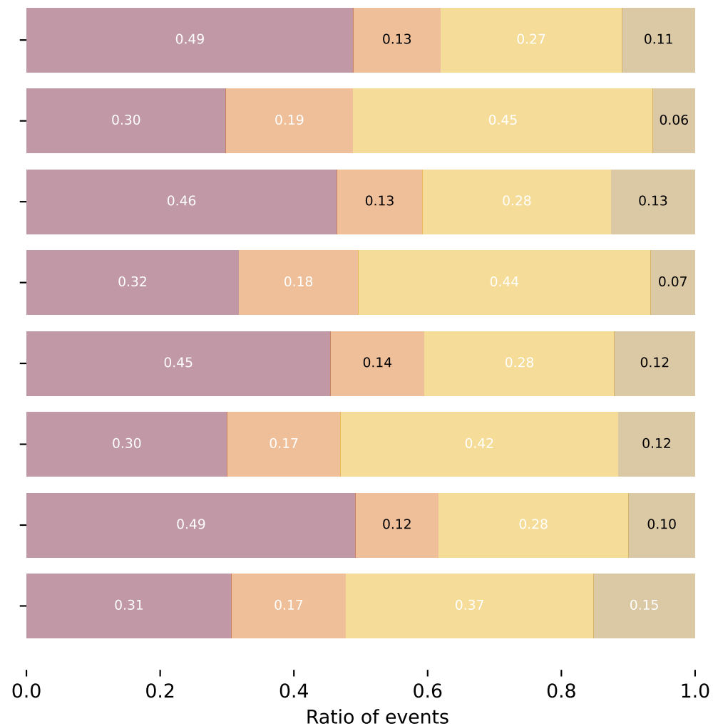
Test set
