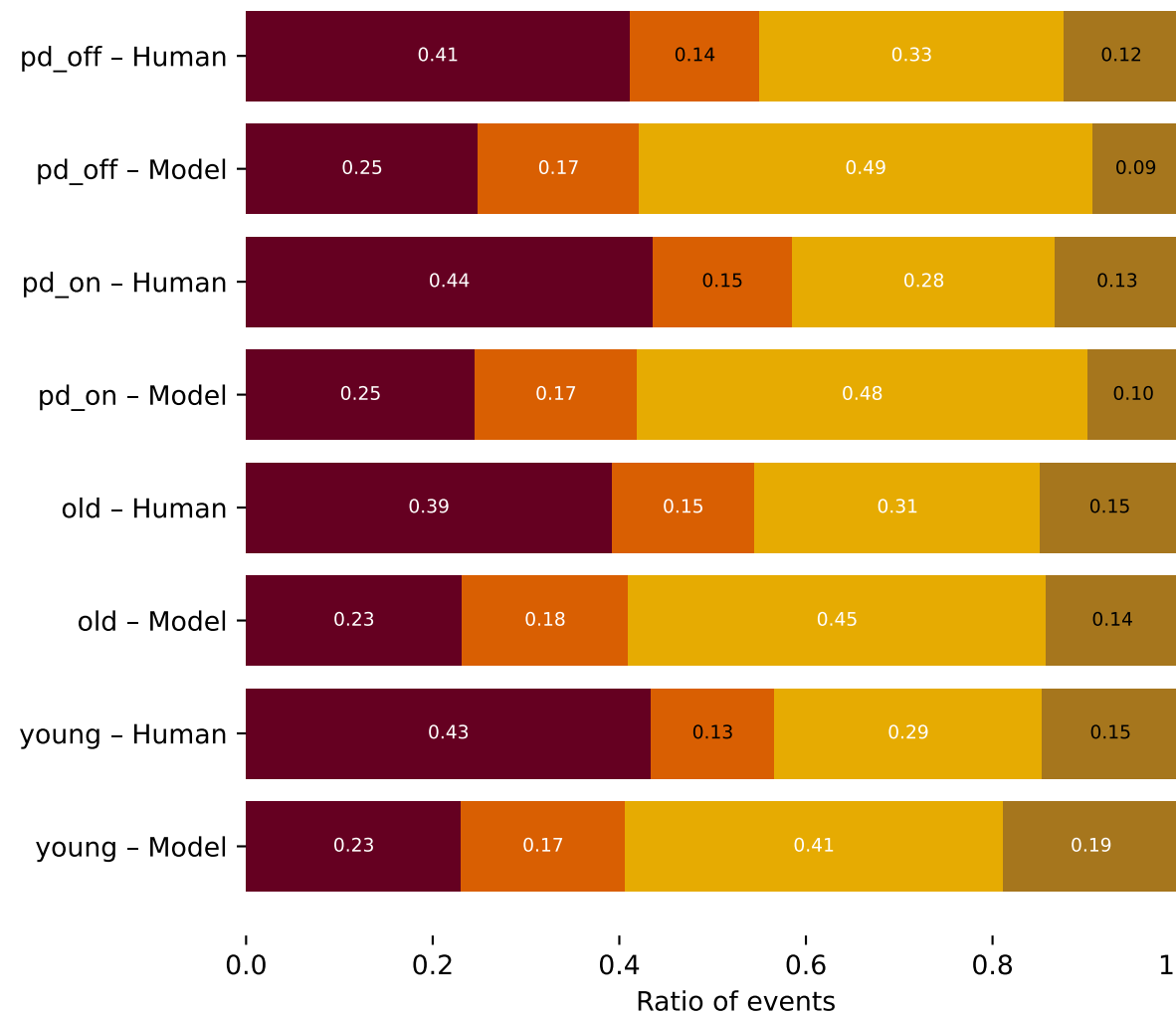
Training set
