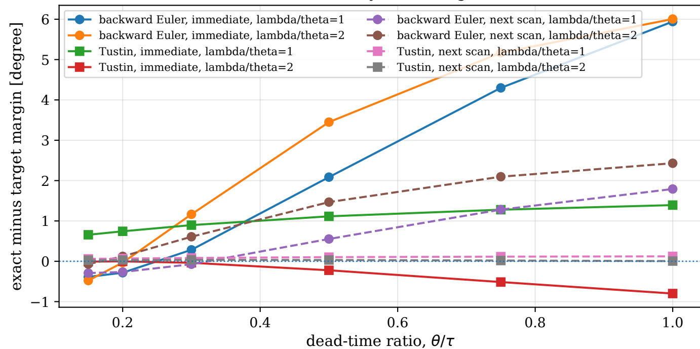
(b) Aggregate over 12 plant/tuning cases
