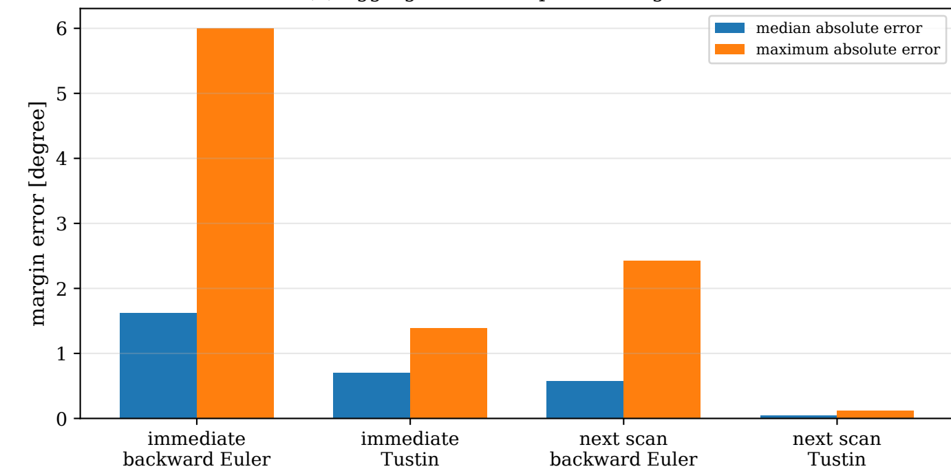
(b) Aggregate over 12 plant/tuning cases
