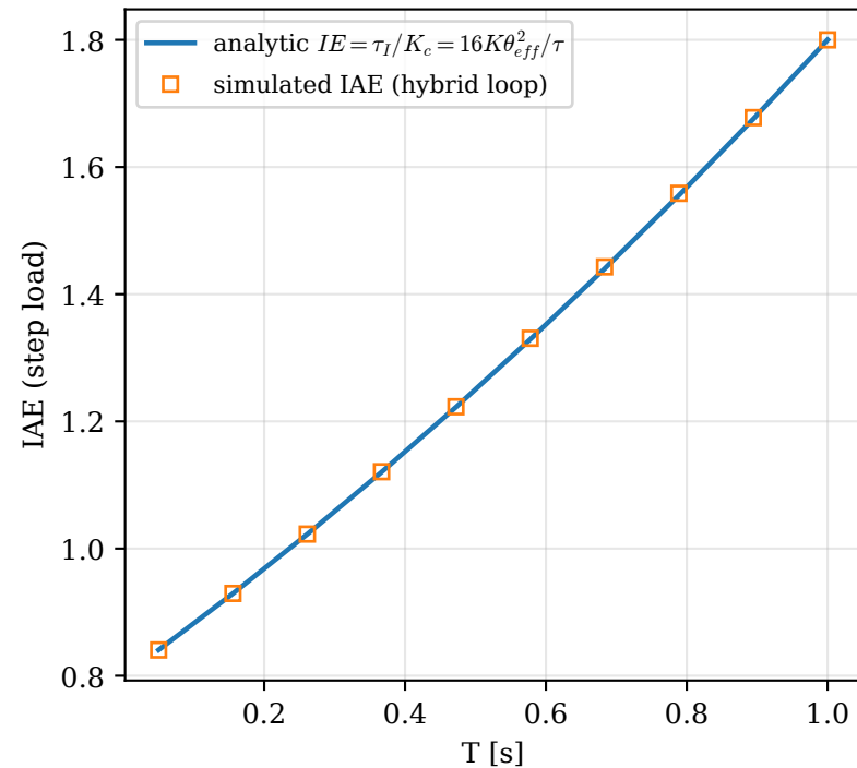
lag-dominant FOPTD \tau=20, \theta=1 : quadratic law
