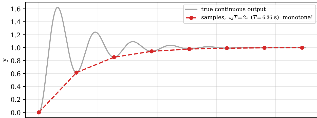
Hidden oscillation, \zeta = 0.15 , \omega_n = 1.0 : digital system sees a first-order response
